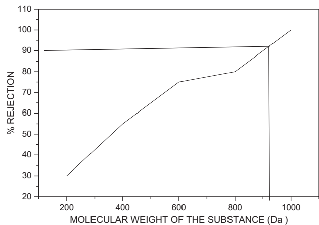
Figure 7 MWCO curve for newly synthesized NF membrane.
