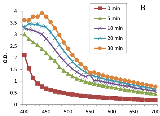
Figure 2B UV-visible spectrum of biosynthesized TE-AgNPs at different time intervals, showed peak at 430 nm.
