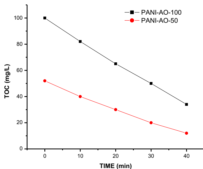
Figure 6 TOC of PANI-AO-100 and PANI-AO-50.
