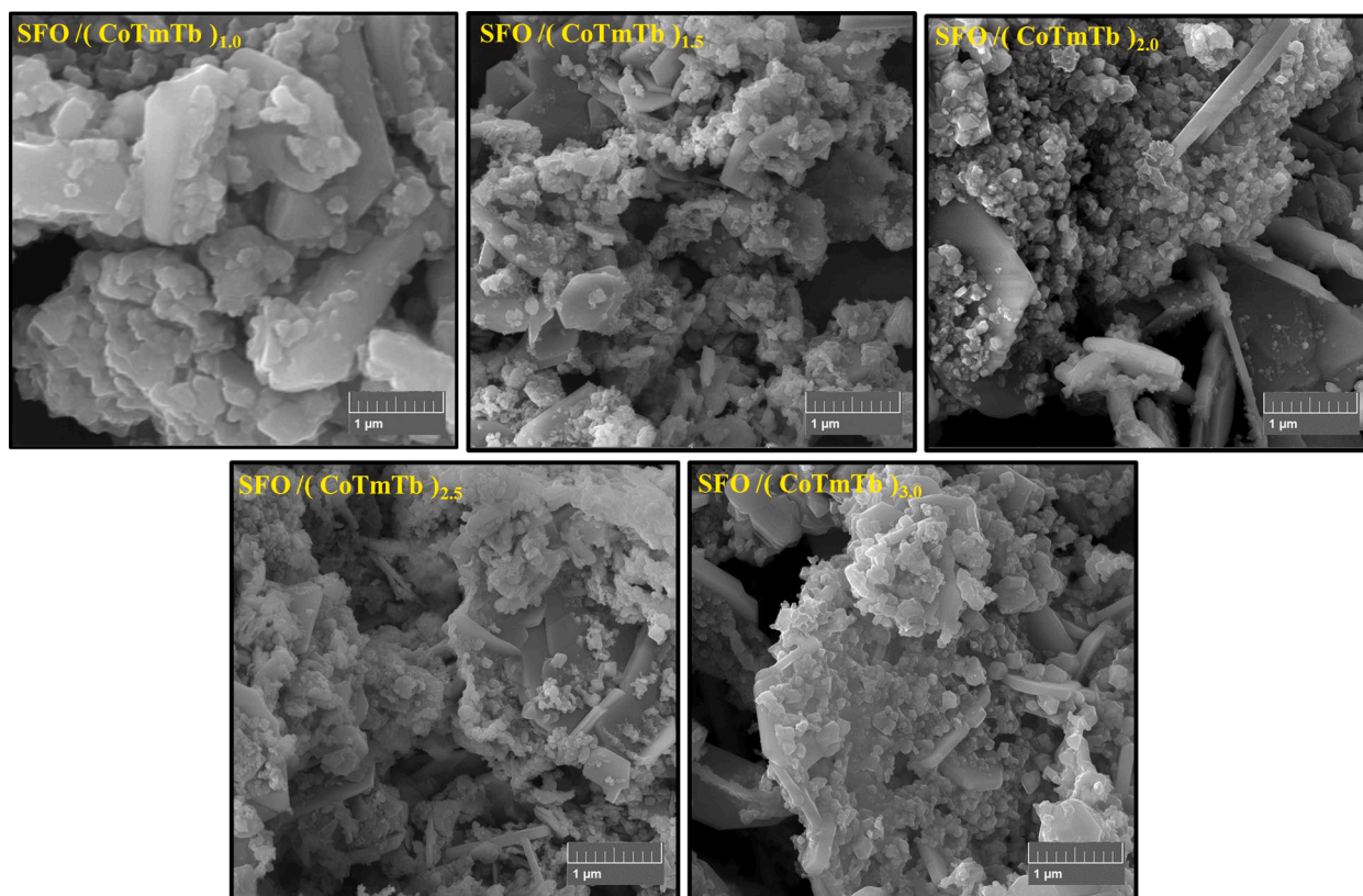
Fig. 2. SEM images of hard/soft SFO/x(CoTmTb) (x ≤ 3.0) NCs.
