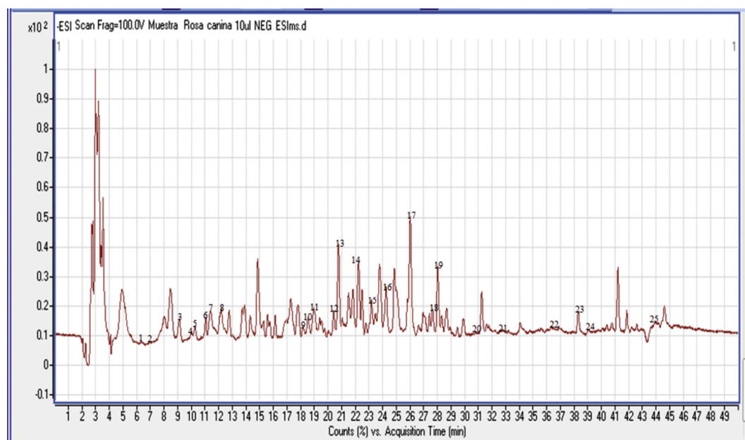
Fig. 4 HPLC-MS-DAD chromatograms of extract of Rosa canina fruits at-ESI mode.
