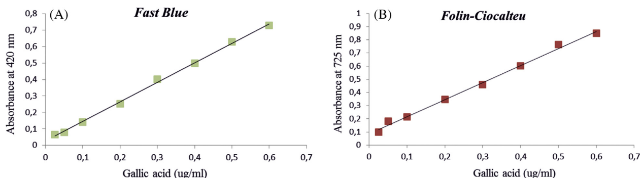
Fig. 1 Calibration curve of total phenolic content (TPC) of ethanolic extract of Rosa canina fruits using fast blue method (1A), and Folin-Ciocalteu (1B).
