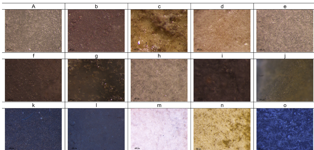
Fig. 2 Optical microscope photographs of TPU membranes with silver salt and ionic liquid additives; a: pure TPU membrane; b: 10 wt.% \text{AgNO}_3 ; c: 20 wt.% \text{AgNO}_3 ; d: 10 wt.% \text{Ag}[\text{PF}_6] ; e: 10 wt.% \text{Ag}[\text{BF}_4] ; f: 10 wt.% \text{Ag}[\text{Tf}_2\text{N}] ; g: 20 wt.% \text{Ag}[\text{PF}_6] ; h: 20 wt.% \text{Ag}[\text{BF}_4] ; i: 20 wt.% \text{Ag}[\text{Tf}_2\text{N}] ; j: 10 wt.% \text{AgNO}_3 + 10% [\text{C}_4\text{mim}][\text{NO}_3] ; k: 10 wt.% \text{Ag}[\text{PF}_6] + 10% [\text{C}_4\text{mim}][\text{PF}_6] ; l: 10 wt.% \text{Ag}[\text{BF}_4] + 10% [\text{C}_4\text{mim}][\text{BF}_4] ; m: 10 wt.% \text{Ag}[\text{Tf}_2\text{N}] + 10% [\text{C}_4\text{mim}][\text{Tf}_2\text{N}] ; n: 10 wt.% \text{AgNO}_3 + 20% [\text{C}_4\text{mim}][\text{NO}_3] ; o: 10 wt.% \text{Ag}[\text{PF}_6] + 20% [\text{C}_4\text{mim}][\text{PF}_6] at 293 K and at atmospheric pressure.
