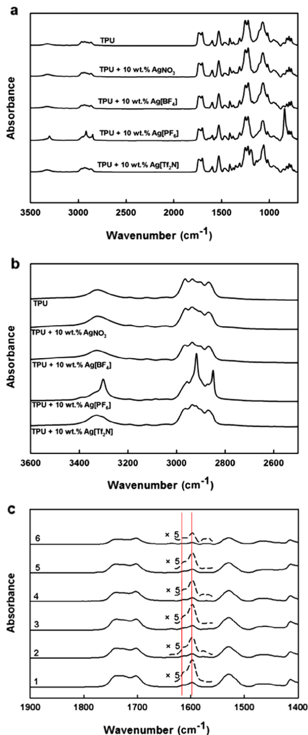
Fig. 4 FTIR of prepared membranes; (a) silver salt membranes; (b) expansion of the N—H and C—H bond stretching region; (c) FTIR before/after membrane separation test, 1 and 2 denote 10 wt.% \text{AgNO}_3 membrane before and after membrane tests, 3 and 4 denote 10 wt.% \text{AgNO}_3 + 10\text{ wt.}\% [\text{C}_4\text{mim}][\text{NO}_3] membrane before and after membrane tests, 5 and 6 denote \text{AgNO}_3 + 10\text{ wt.}\% [\text{C}_4\text{mim}][\text{TF}_2\text{N}] membrane before and after membrane tests.
