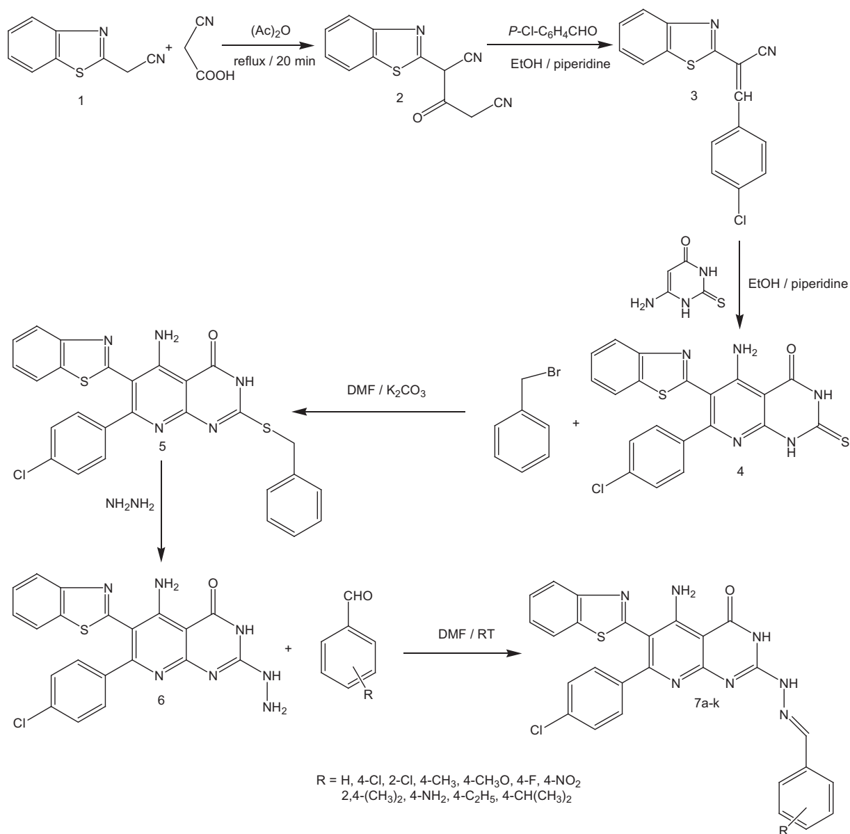
Scheme 1 Synthesis pathway of benzothiazole pyrimidine derivatives.
