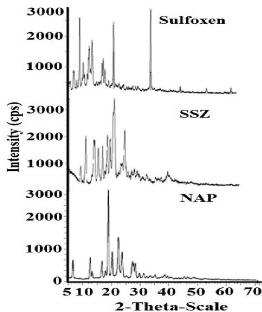
Fig. 5 XRPD patterns of the SSZ, NAP and Sulfoxen complex.
