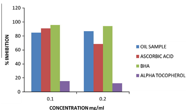
Figure 1 % Inhibition of DPPH free radical scavenging activity of essential oils of L. aestuans . *% Inhibition of oil and reference standards.
