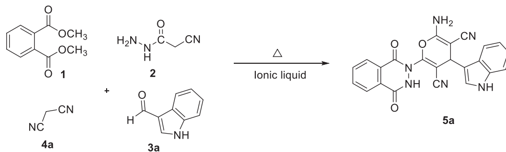
Scheme 1 with the incorrect structure of compound 3a-c:
