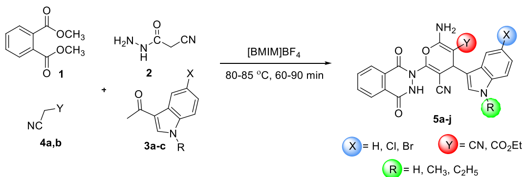
Scheme 1 with the incorrect structure of compound 3a-c:
