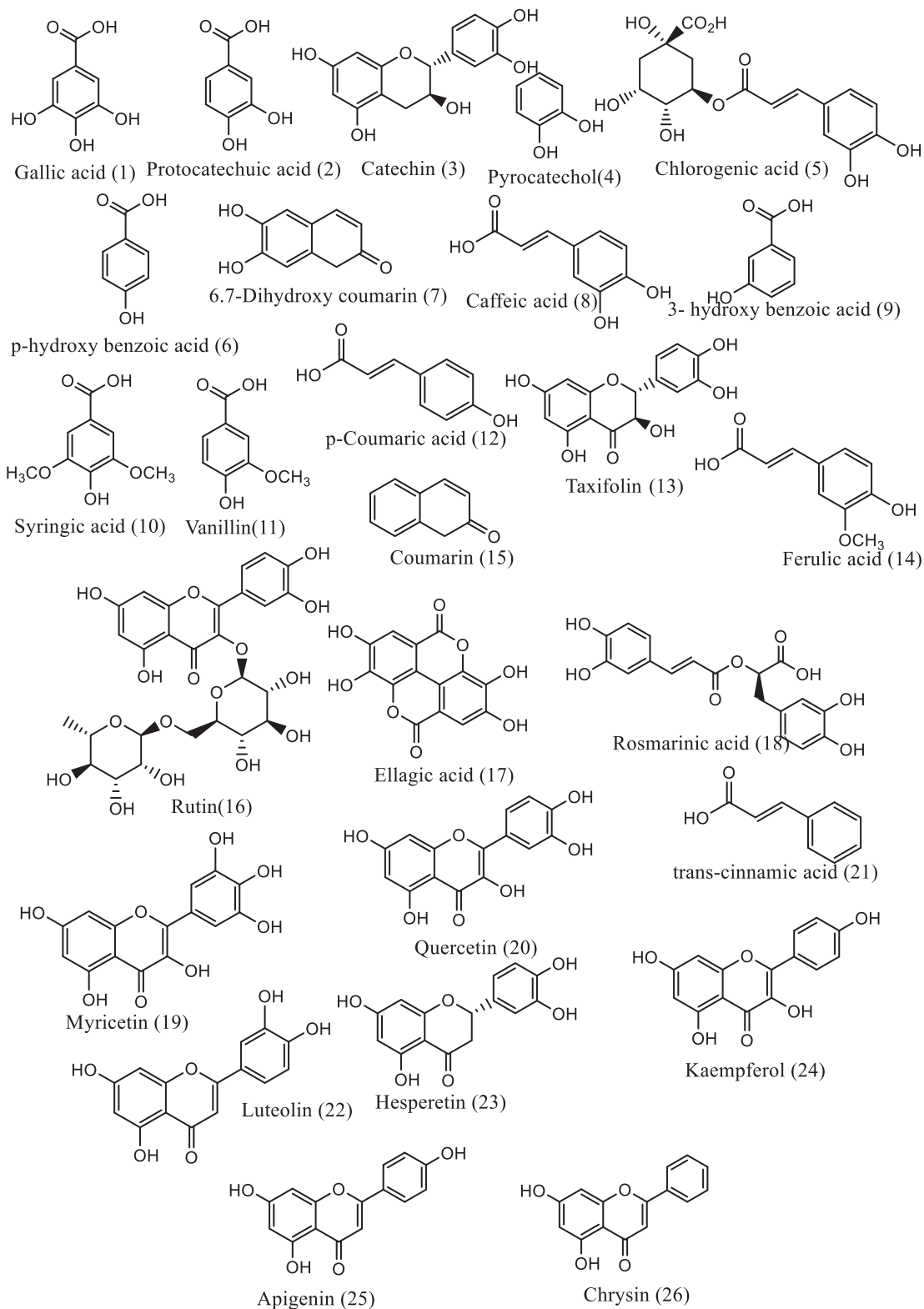
Fig. 1 Structures of identified phenolic compounds in the plant extracts.
