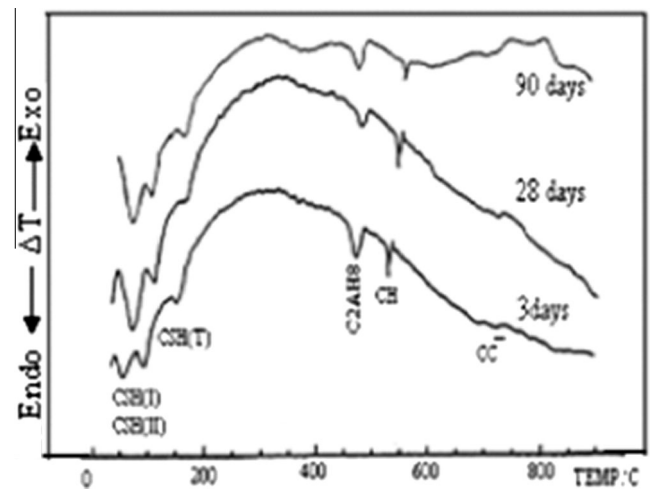
Figure 6 The DTA thermogram of the hardened cement pastes of Mix (M-e) cured up to 90 days.
