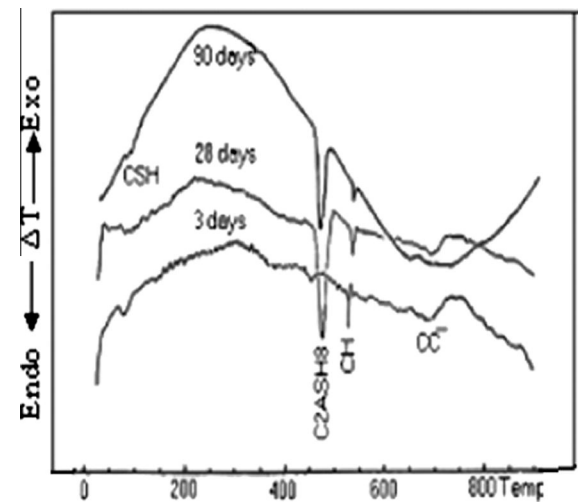
Figure 5 The DTA thermogram of the hardened cement paste Mix (M control) cured up to 90 days.
