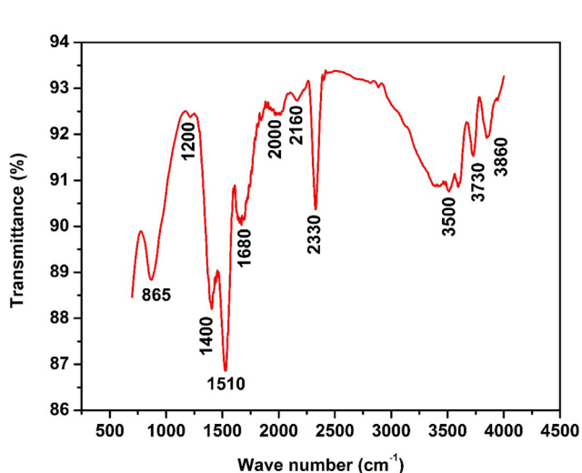
Fig. 6 The FTIR spectrum of biosynthesized ZnO NP's.
