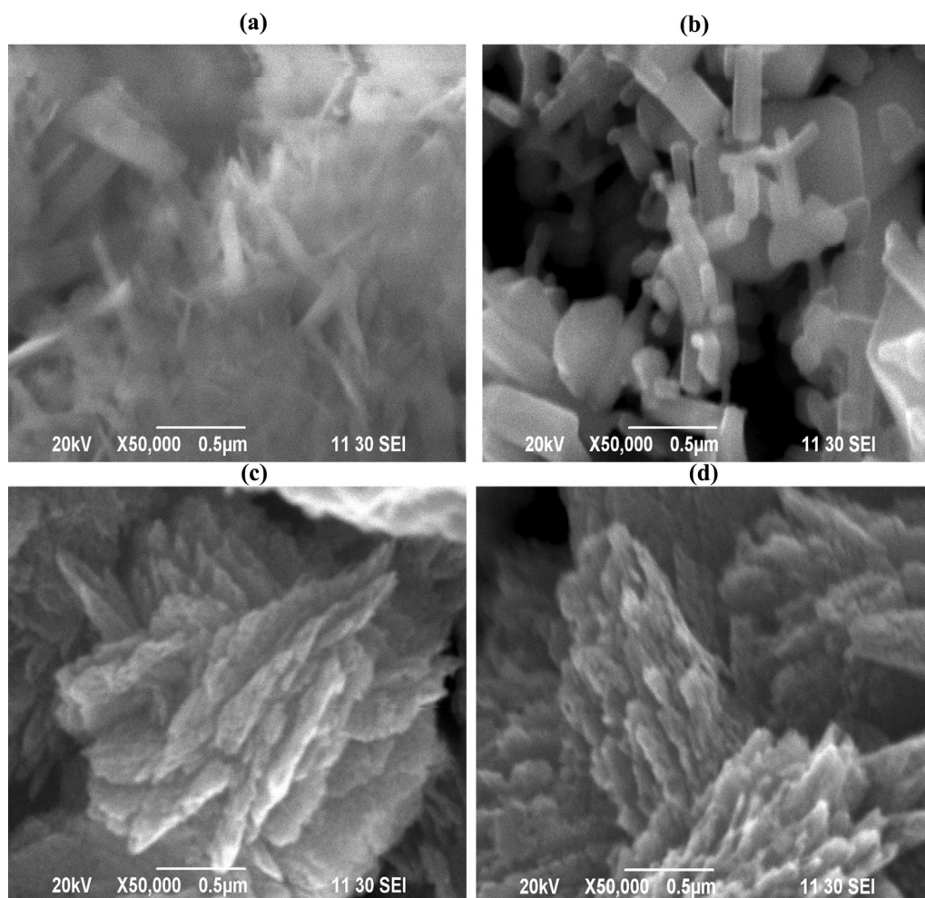
Fig. 1 SEM images of (a) ZnO via sol-gel with 1 % SDS, (b) ZnO via sol-gel with 7 % Triton X-100, (c) ZnO from synthesized \text{ZnCO}_3 at 300 °C and (d) ZnO from commercial \text{ZnCO}_3 at 300 °C.
