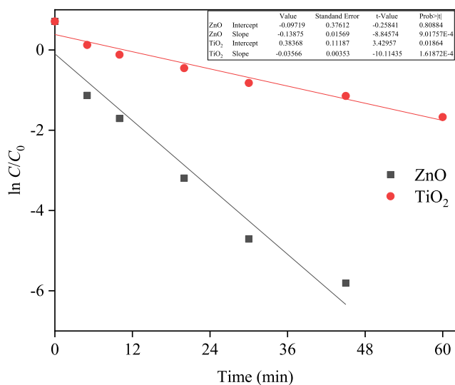
Fig. 3 A plot of \ln C/C_0 vs time for calculating rate constant ( k ) of degradation of RB in presence of nanorod-ZnO and commercial \text{TiO}_2 under solar irradiation. [\text{RB}] = 2.00 \times 10^{-5} \text{ M} ; Solution pH = 7.8.
