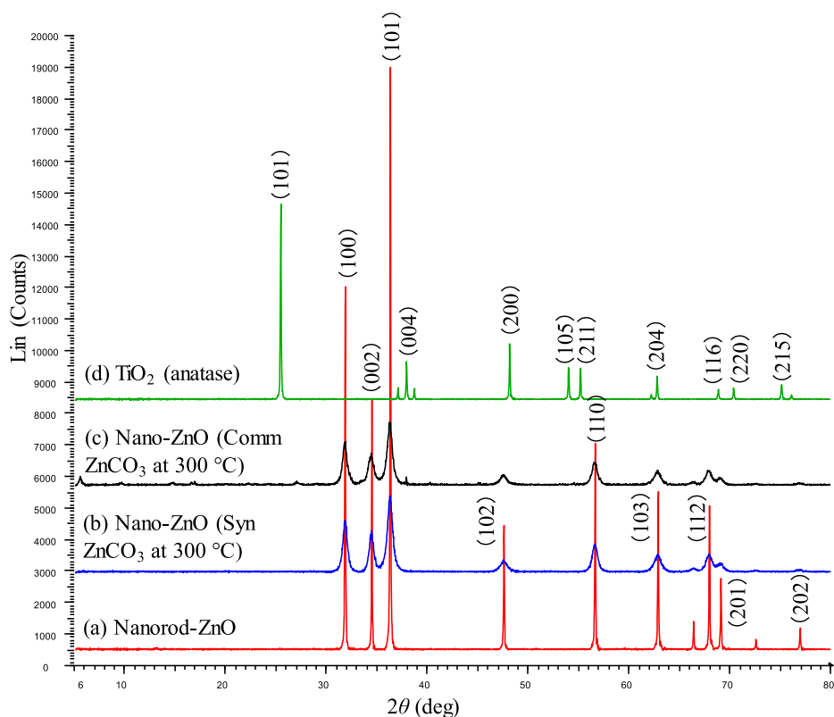
Fig. 2 XRD spectral pattern of (a) nanorod-ZnO, (b) nano-ZnO (synthesized \text{ZnCO}_3 at 300 °C), (c) nano-ZnO (commercial \text{ZnCO}_3 at 300 °C) and (d) commercial \text{TiO}_2 (anatase).
