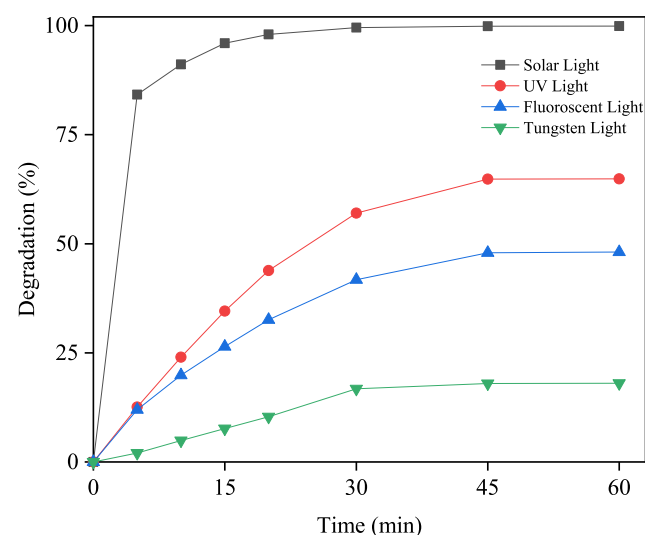
Fig. 5 Degradation (%) of RB in the presence of 0.01 g/50 mL nanorod ZnO under solar, UV, fluorescent and tungsten filament light irradiation. [RB] = 2.00 \times 10^{-5} M; Solution pH = 7.8.
