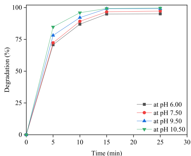
Fig. 4 Effect of solution pH on degradation of RB with 0.01 g/50 mL nanorod-ZnO under solar light irradiation. [RB] = 2.00 \times 10^{-5} M.
