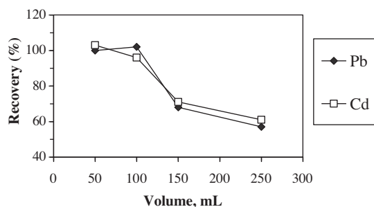
Figure 3 Effect of sample volume on the recovery of Pb(II) and Cd(II).
