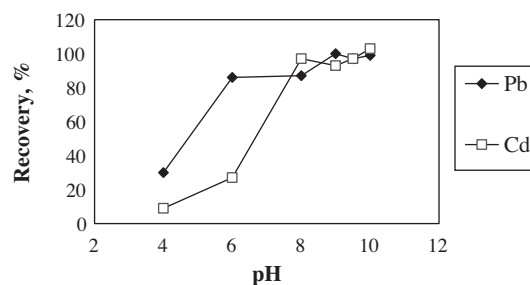
Figure 2 Effect of pH on the recovery of Pb(II) and Cd(II) on a column filled with the impregnated resin (sample volume: 50 mL, eluent: 20 mL of 2 mol L -1 HNO 3 ).
