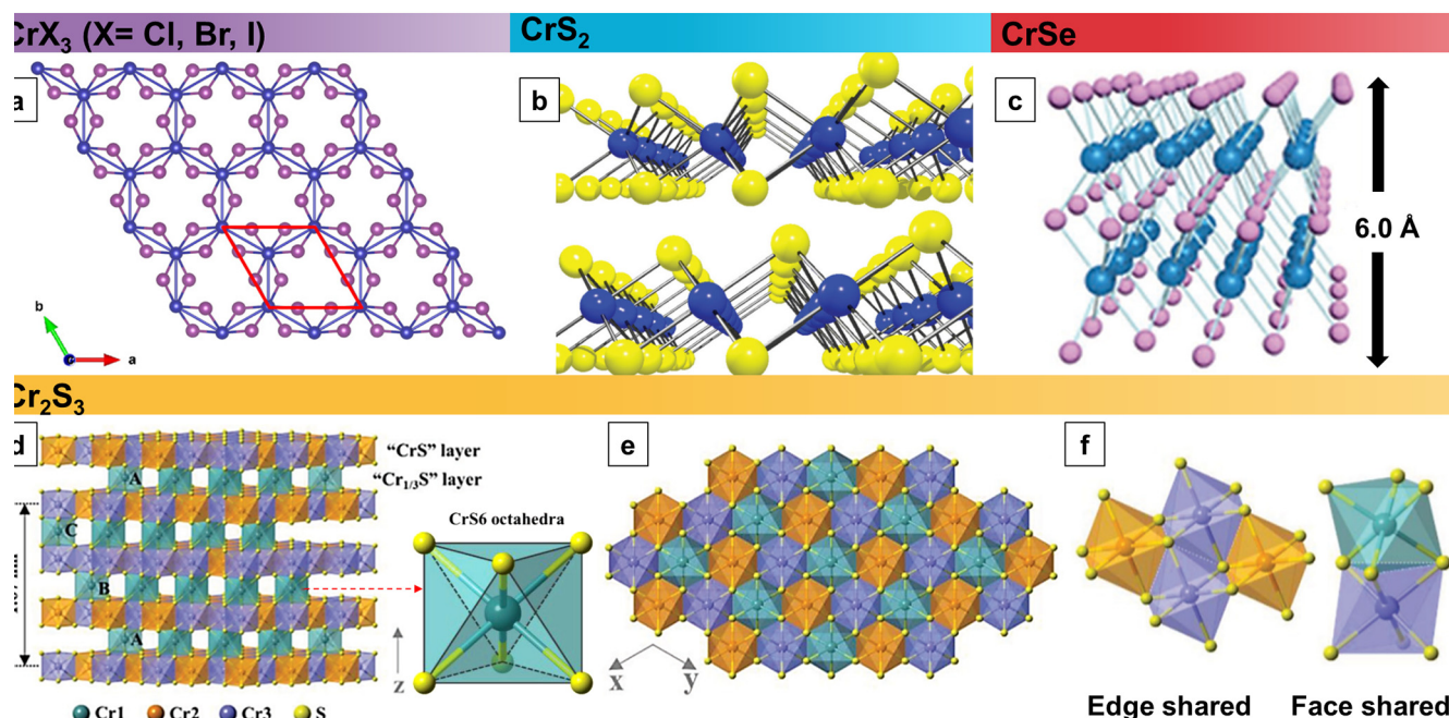
Fig. 2 (a) Atomistic structure of monolayer \text{CrX}_3 ( \text{X} = \text{Cl, Br, or I} ). (a) Top view of a single layer. Reproduced with permission from Ref. (Webster and Yan, 2018) Copyright 2018, American Physical Society. (b) Single-layer \text{CrS}_2 with 2H (top) and 1T (bottom) structures. Cr and S are represented by the blue and yellow balls, respectively. Reprinted from Ref. (Zhuang et al., 2014) [APPLIED PHYSICS LETTERS 104, 022,116 (2014)] with the permission from AIP Publishing (c) Structural model of a \text{CrSe} crystal. Reproduced with permission from Ref. (Zhang et al., 2019). Copyright 2019, John Wiley and Sons (d-f) Structural models of rhombohedral \text{Cr}_2\text{S}_3 . (d) Perspective view and (e) top view showing the periodic stack of the fully filled "CrS" layer and partially filled "Cr 1/3 S" layer. The stacking along the z-direction with an A–B–C sequence induces a rhombohedral \text{Cr}_2\text{S}_3 . Blue, orange, and purple balls represent Cr atoms with different occupancies in the structure. Yellow balls denote S atoms. The entire structure is composed of \text{CrS}_6 octahedras, in which (f) interlayer octahedras are connected by faces, whereas the intralayer octahedras are connected by edges. Reproduced with permission from Ref. (Zhou et al., 2019;29(3):1805880.). Copyright 2018, John Wiley and Sons.
