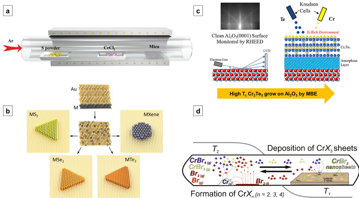
Fig. 5 Different methods for fabricating the 2D Cr-based materials. (a) Schematic for CVD synthesis of ultrathin \text{Cr}_2\text{S}_3 flakes on two stacked mica sheets with \text{CrCl}_2 and S as the co-evaporation sources. Reproduced with permission from Ref. (Zhou et al., 2019;29(3):1805880.). Copyright 2018, John Wiley and Sons. (b) A general approach for synthesizing thin layers of 2D binary compounds. Reproduced with permission from Ref. (Shivayogimath et al., 2019) Creative Commons CC BY, Springer Nature (c) Schematics of high- T_c \text{Cr}_2\text{Te}_3 thin films grown on \text{Al}_2\text{O}_3 via molecular beam epitaxy. Reprinted (adapted) with permission from Ref. (Li et al., 2019) [ACS Appl. Nano Mater. 2019, 2, 11, 6809–6817], copyright [2019] American Chemical Society. (d) Scheme for the one-step synthesis and vapor transport of \text{CrX}_3 ( X = \text{Br}, \text{I} ) micro- and nanosheets. Reproduced with permission from Ref. (Grönke et al., 2019). Creative Commons License, John Wiley and Sons.
