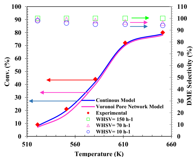
Fig. 10 Comparison of MeOH conversion-temperature results obtained from continuous and Voronoi Pore Network models versus experimental results and DME selectivity (%) at different T_{inlet} and WHSV.
