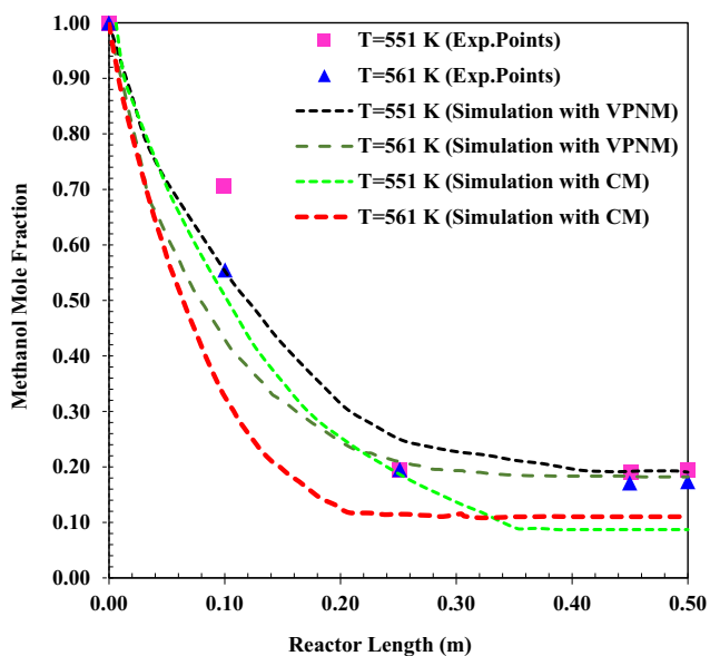
Fig. 4 MeOH mole fraction as a function of reactor length at different inlet temperature (VPNM Simulation (Li et al., 2021c), (Exp.Points (Bercic and Levec, 1993).
