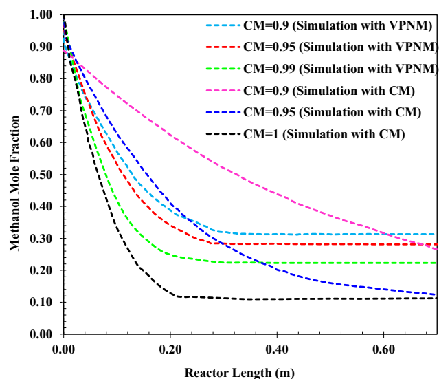
Fig. 7 MeOH mole fraction as a function of reactor length at q = 4.34 L/h and at T_0 = 561 K for different CM. (VPNM Simulation (Li et al., 2021c).
