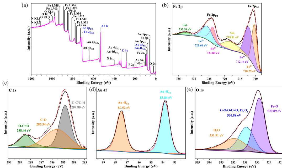
Figure 3. XPS spectra of \text{Fe}_3\text{O}_4/\alpha\text{-Fe}_2\text{O}_3/\text{Au} NCs nanocomposites: (a) Overview spectrum, (b) Fe 2p, (c) C 1s, (d) Au 4f, and (e) O 1s.
