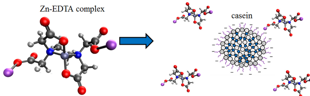
Fig. 14 Diagram of the state of dispersion of casein micelles in the presence of Zn-EDTA molecules.
