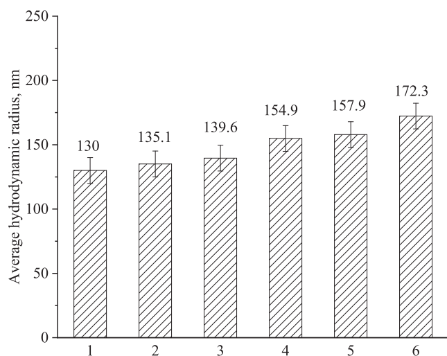
Fig. 4 Average hydrodynamic radius of dispersed phase particles of milk samples: 1-without impurities, 2-enriched with Zinc lysinoriboflavin, 3- Zn-EDTA, 4- Zinc asparaginate, 5- Zinc lactate, 6- Zinc sulfate.
