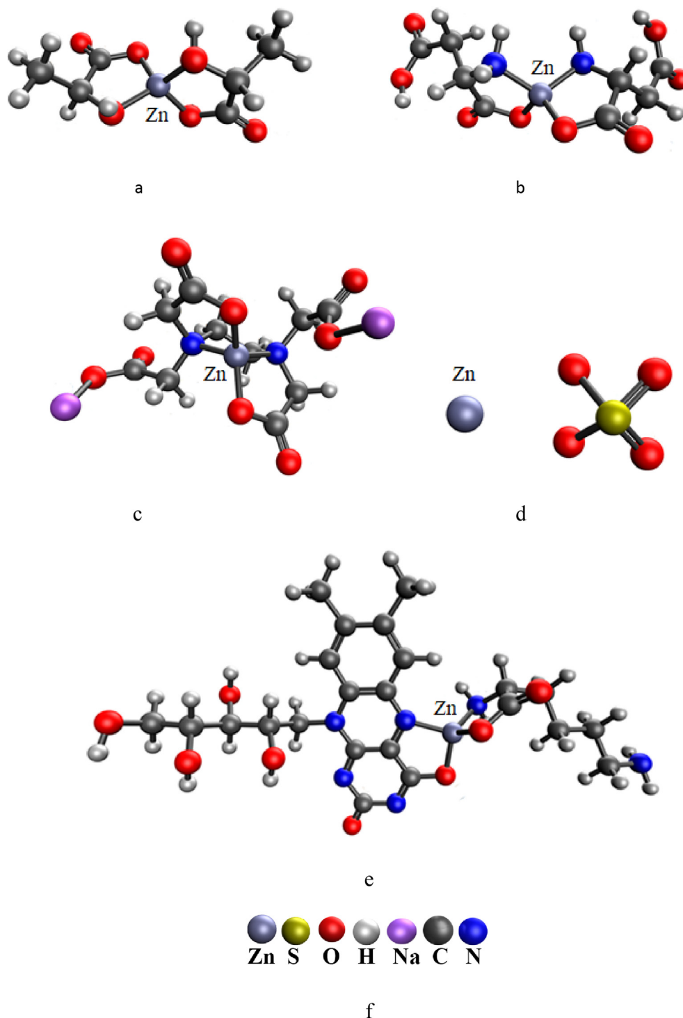
Fig. 2 Models of molecules of Zinc -containing compounds: a) Zinc lactate, b) Zinc asparaginate c) Zinc chelate complex molecule with EDTA, d) Zinc sulfate, e) lysinatoriboflavin Zinc sulfate f) models legend.
