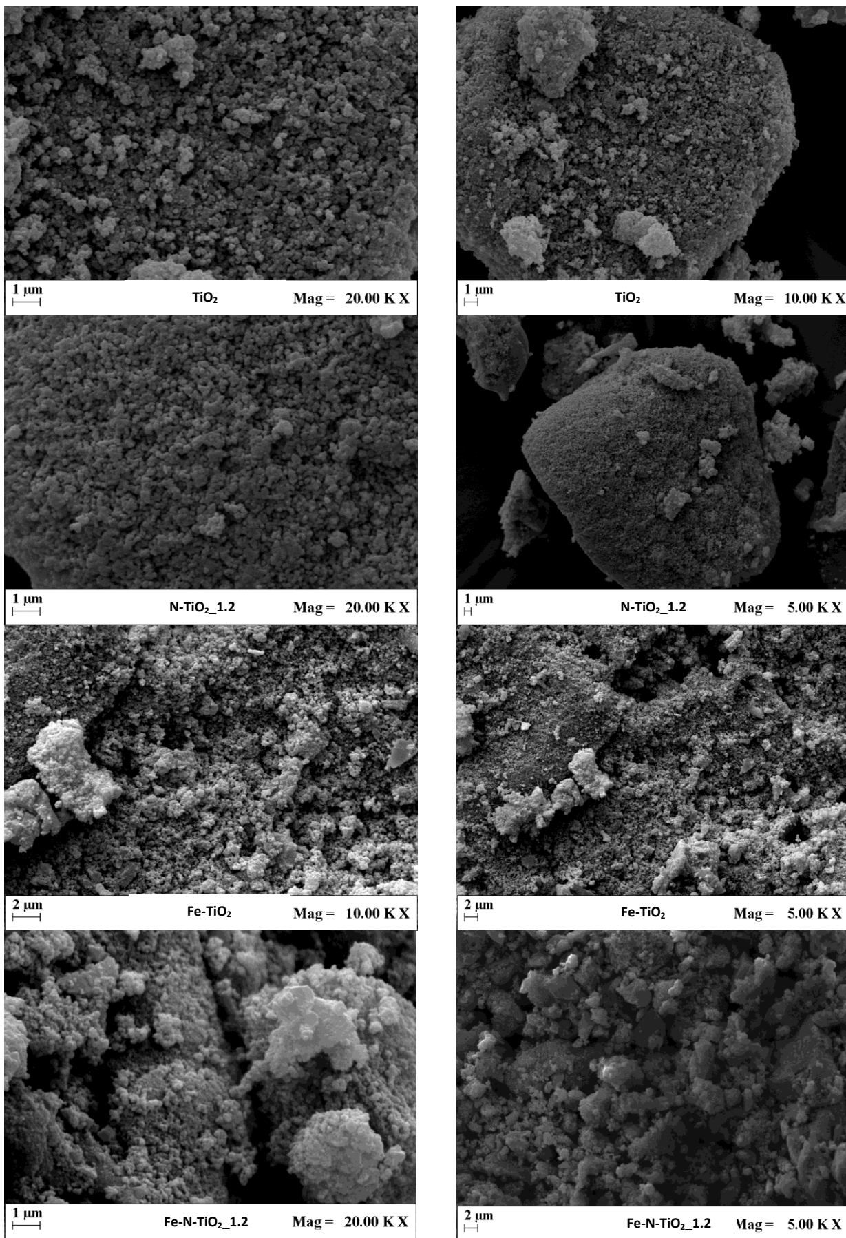
Figure S1: FESEM images of TiO 2 , N-TiO 2_1.2 , Fe-TiO 2 and Fe-N-TiO 2_1.2 photocatalysts.
