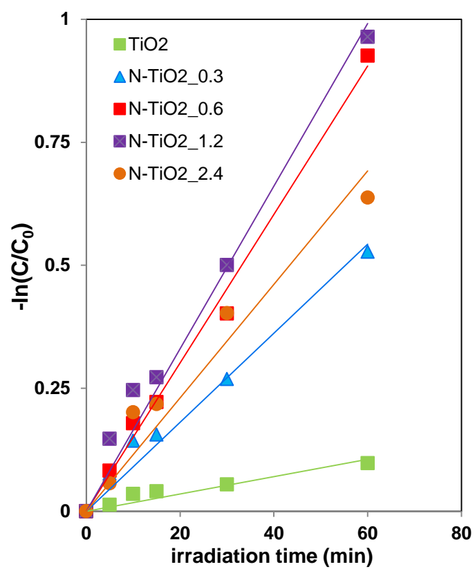
Figure S2: -\ln(C/C_0) vs irradiation time for AO7 discoloration using TiO 2 , N-TiO 2 _0.3, N-TiO 2 _0.6, N-TiO 2 _1.2 and N-TiO 2 _2.4 samples.
