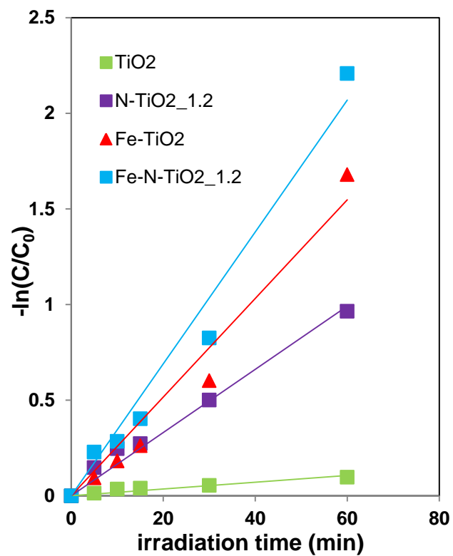
Figure S3: -\ln(C/C_0) vs irradiation time for AO7 discoloration for TiO 2 , N-TiO 2 _1.2, Fe-TiO 2 and Fe-N-TiO 2 _1.2 samples
