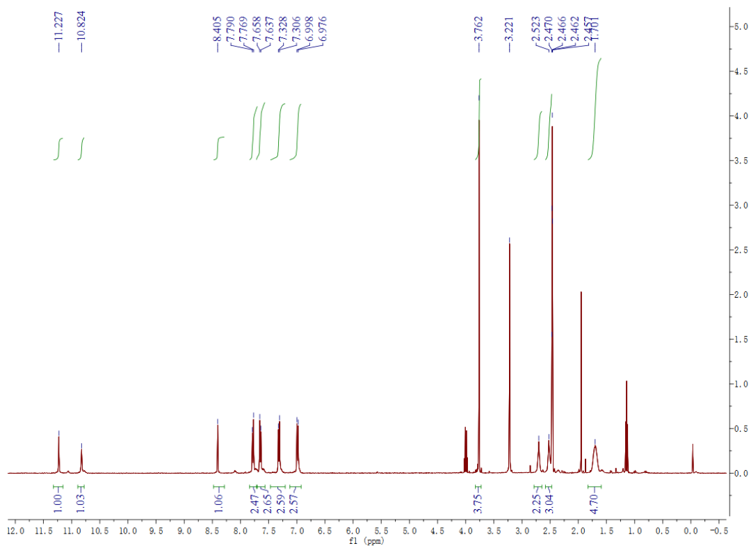
Figure S14. 1 H NMR of compound 7e
