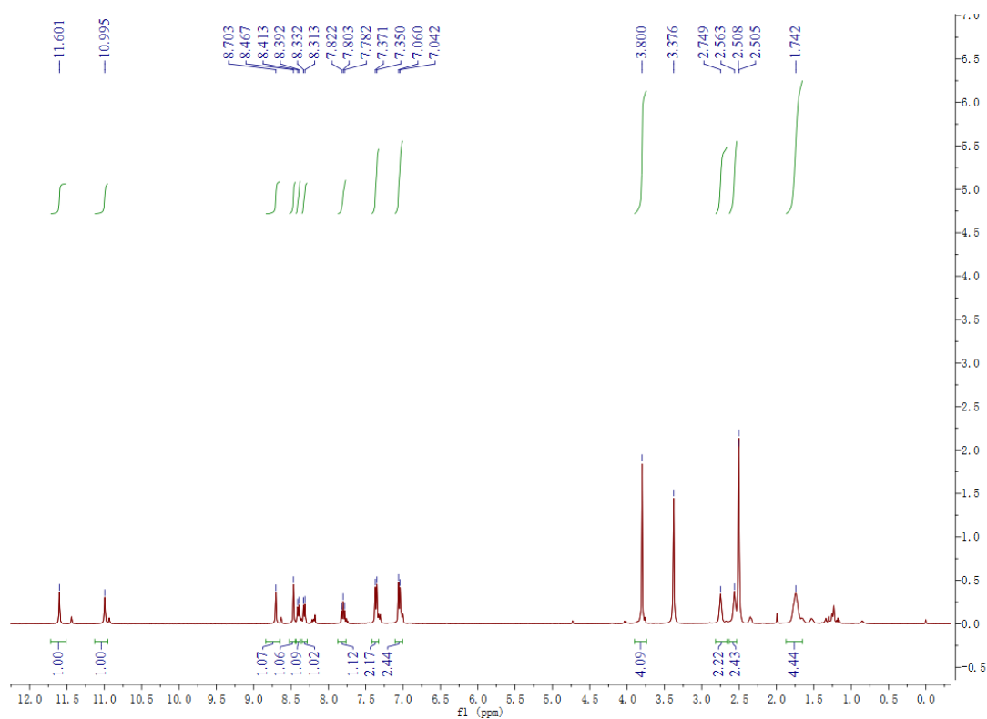
Figure S29. 1 H NMR of compound 7j
