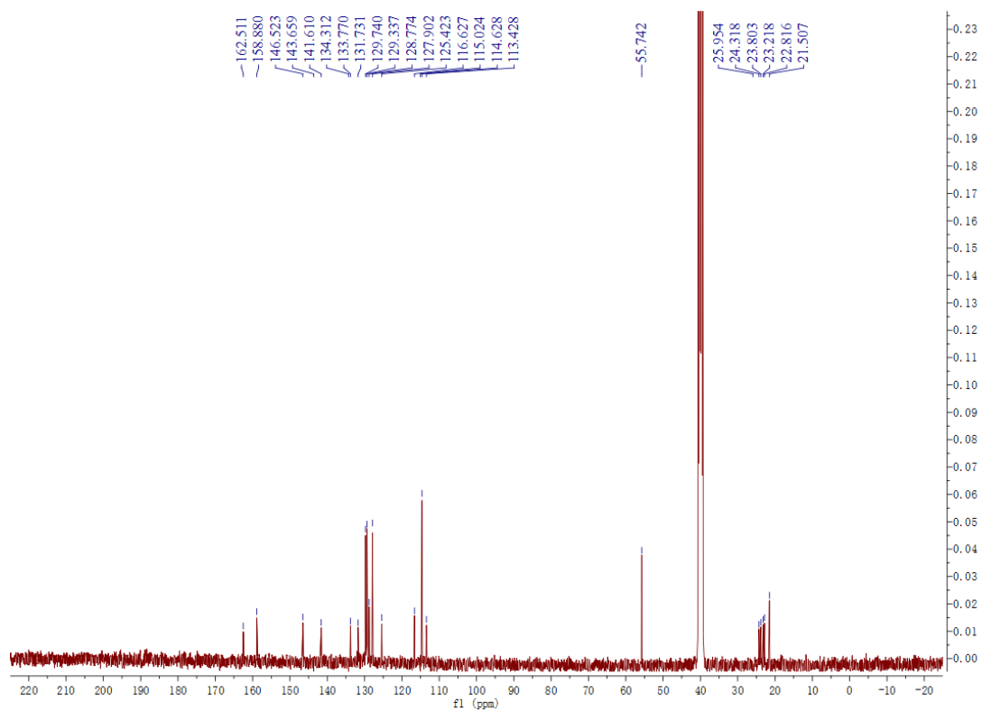
Figure S21. ^{13}\text{C} NMR of compound 7g
