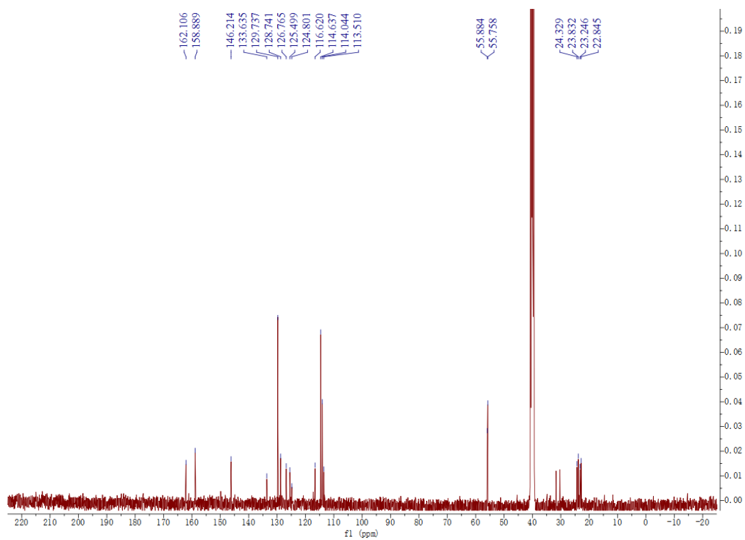
Figure S6. ^{13}\text{C} NMR of compound 7b
