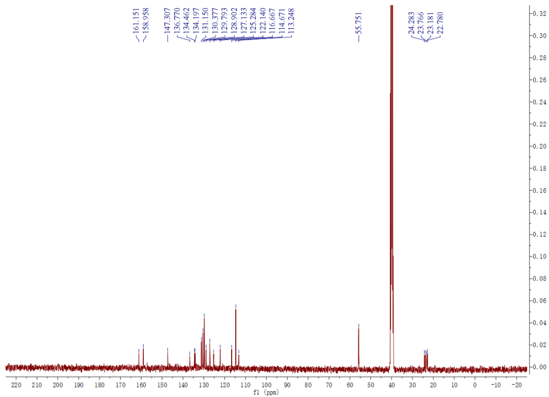
Figure S45. ^{13}\text{C} NMR of compound 7o
