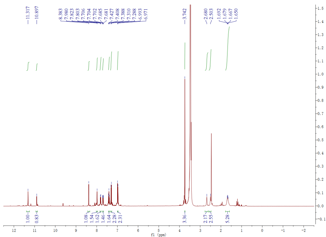
Figure S44. 1 H NMR of compound 7o
