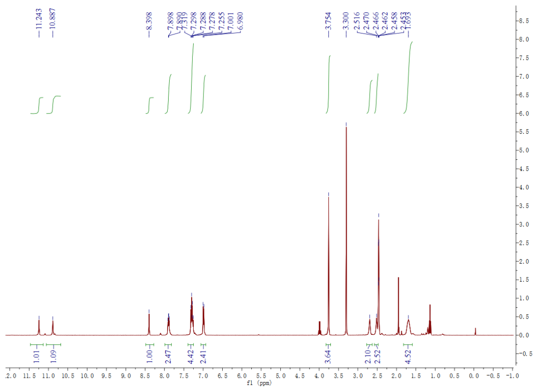
Figure S2. ^1\text{H} NMR of compound 7a
