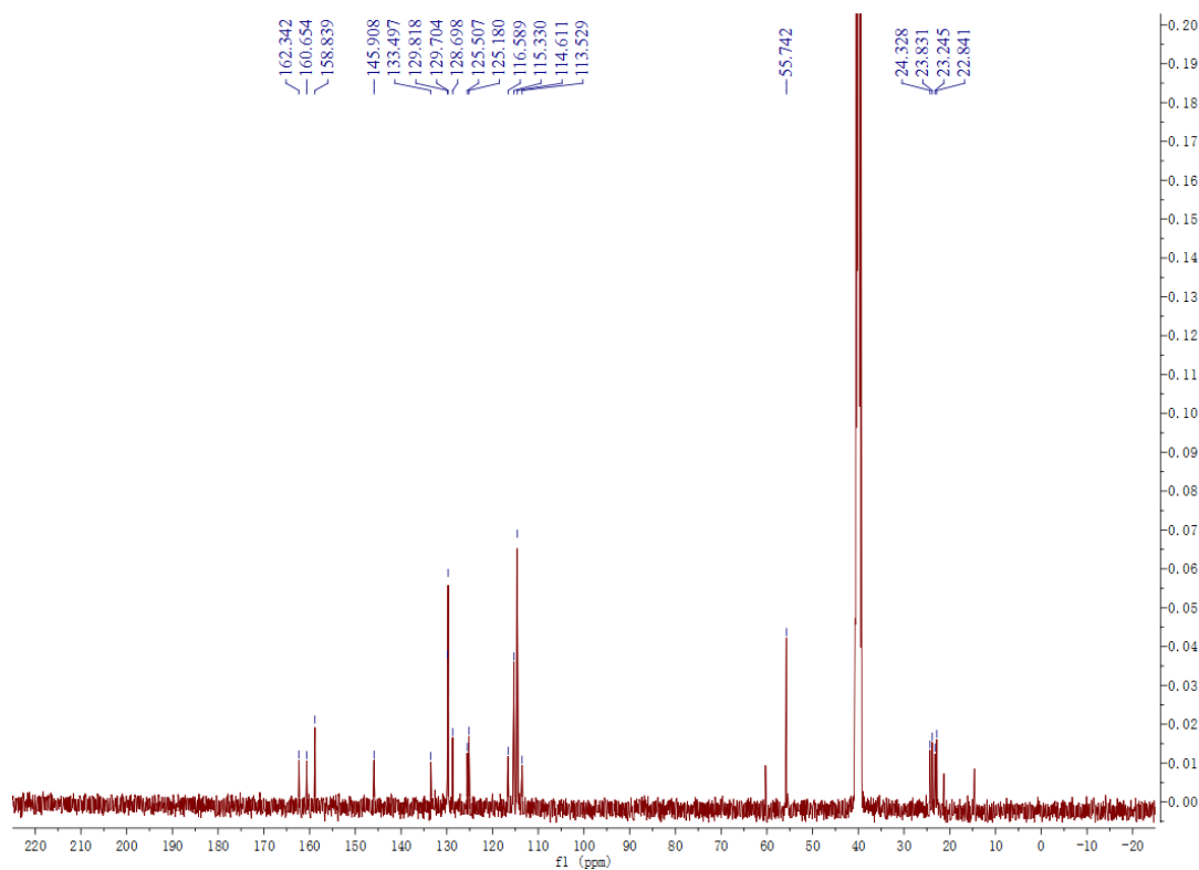
Figure S42. 13 C NMR of compound 7n
