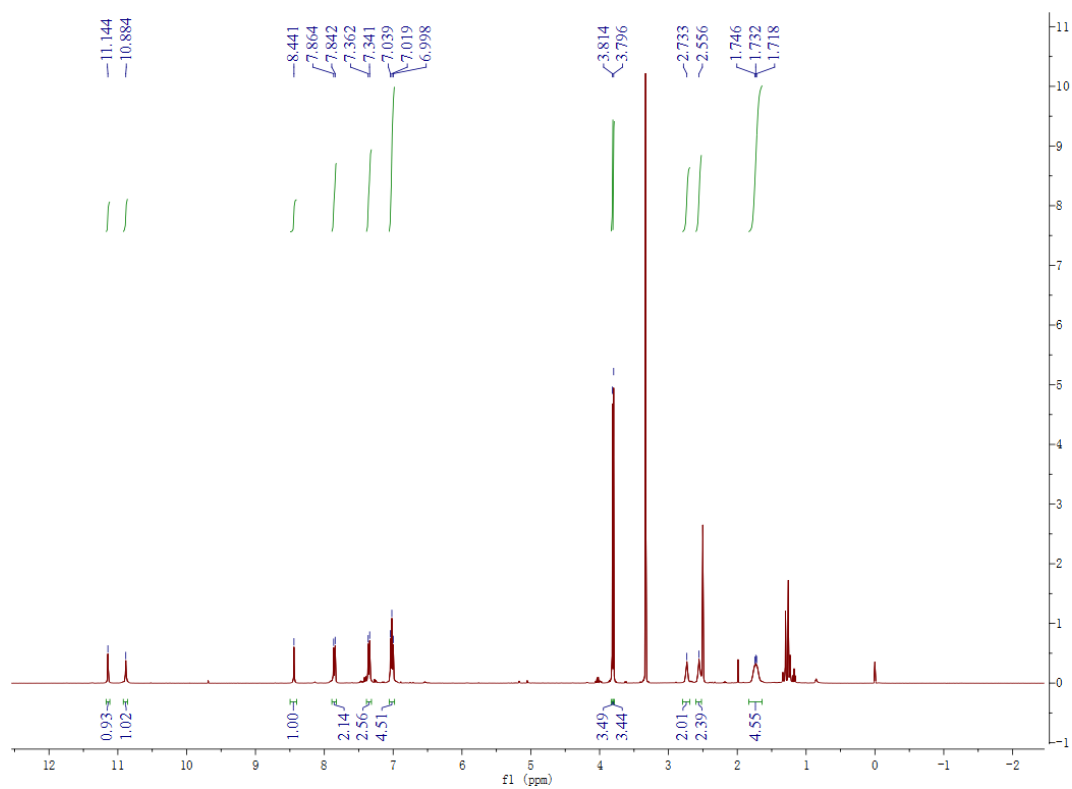
Figure S5. ^1\text{H} NMR of compound 7b
