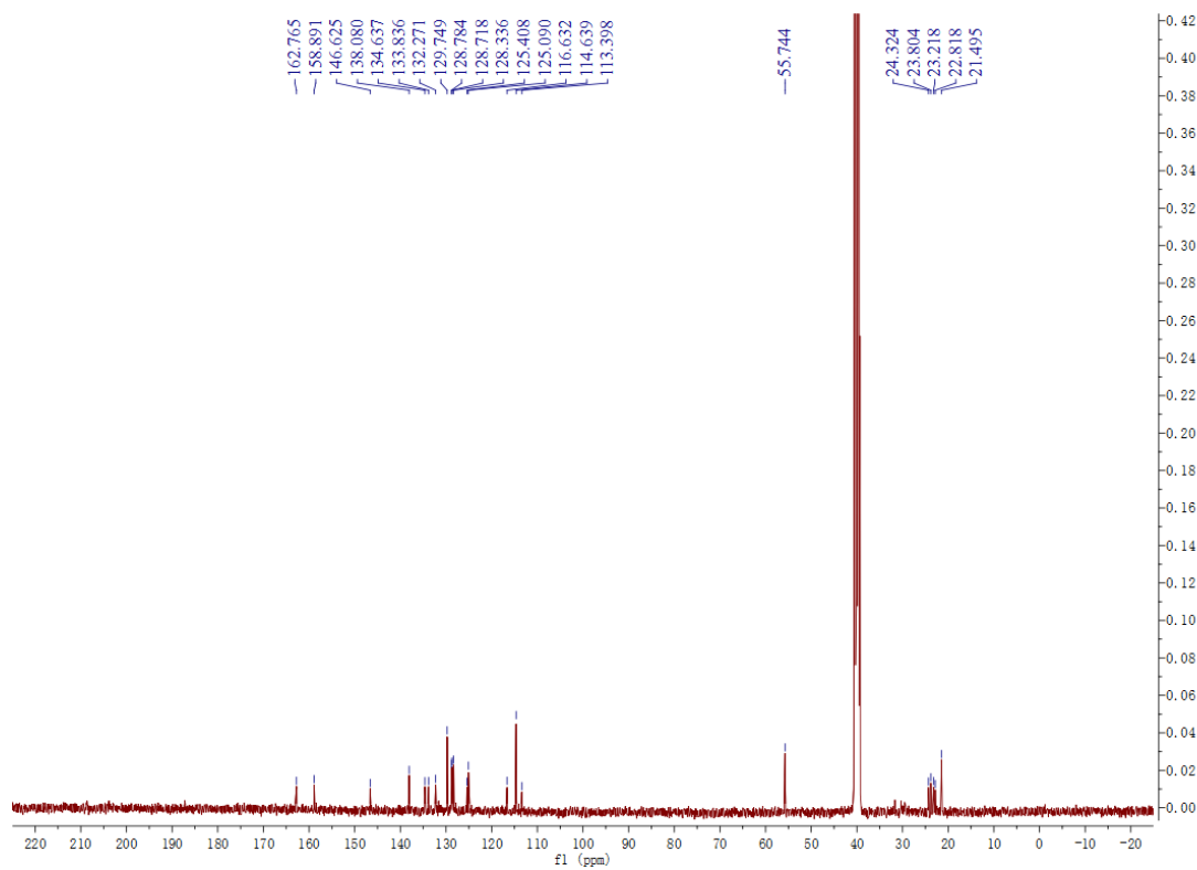
Figure S24. 13 C NMR of compound 7h
