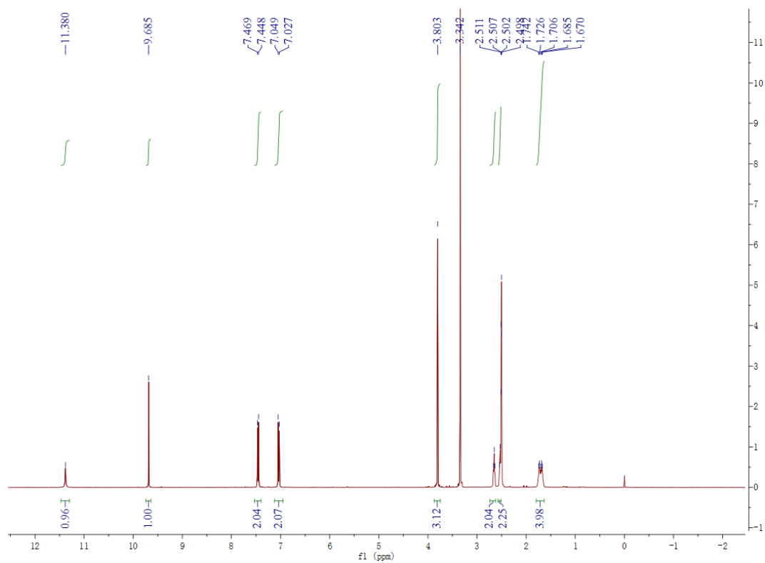
Figure S1. ^1\text{H} NMR of compound 5
