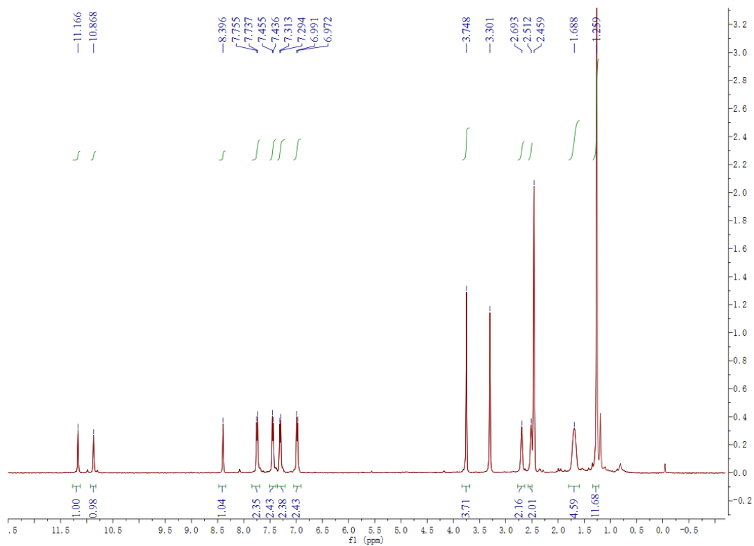
Figure S8. ^1\text{H} NMR of compound 7c
