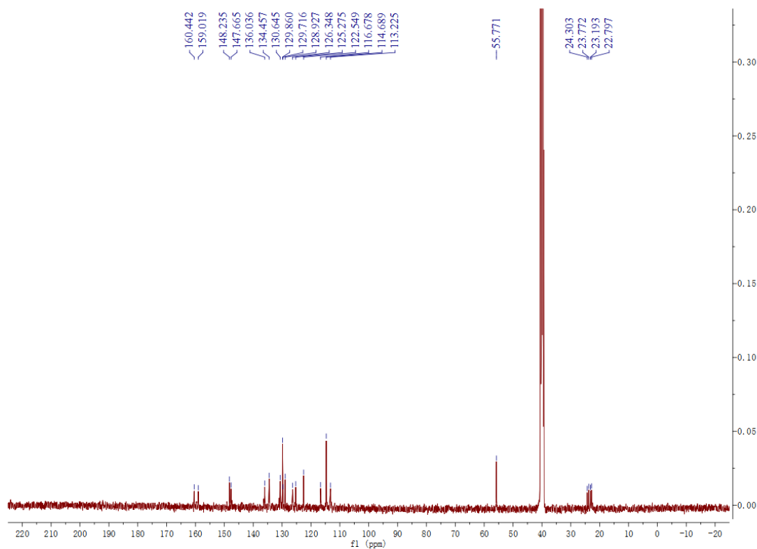
Figure S30. 13 C NMR of compound 7j
