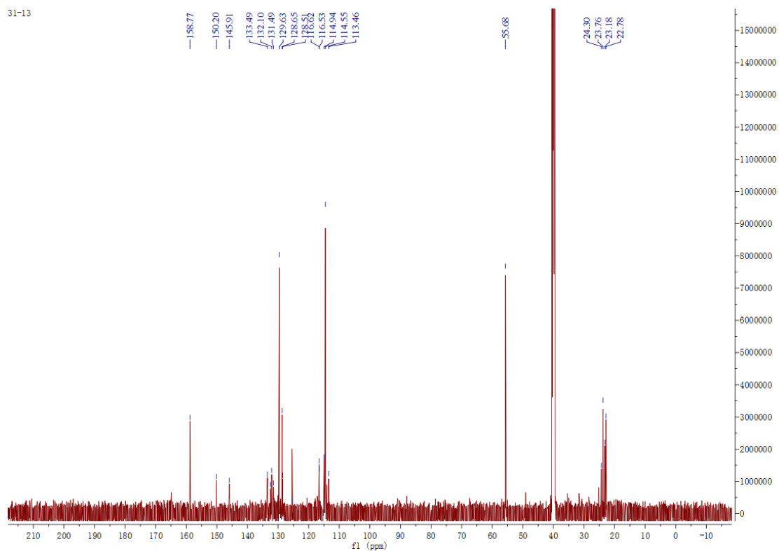
Figure S36. 13 C NMR of compound 7I
