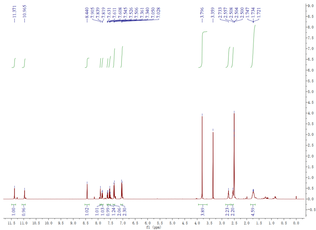
Figure S26. ^1\text{H} NMR of compound 7i
