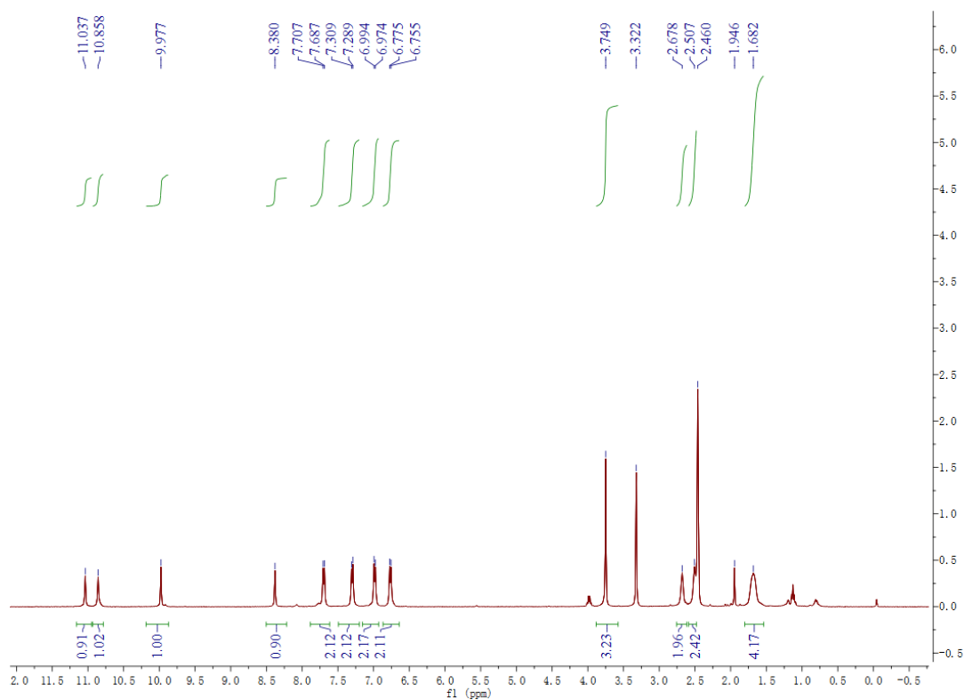
Figure S41. 1 H NMR of compound 7n
