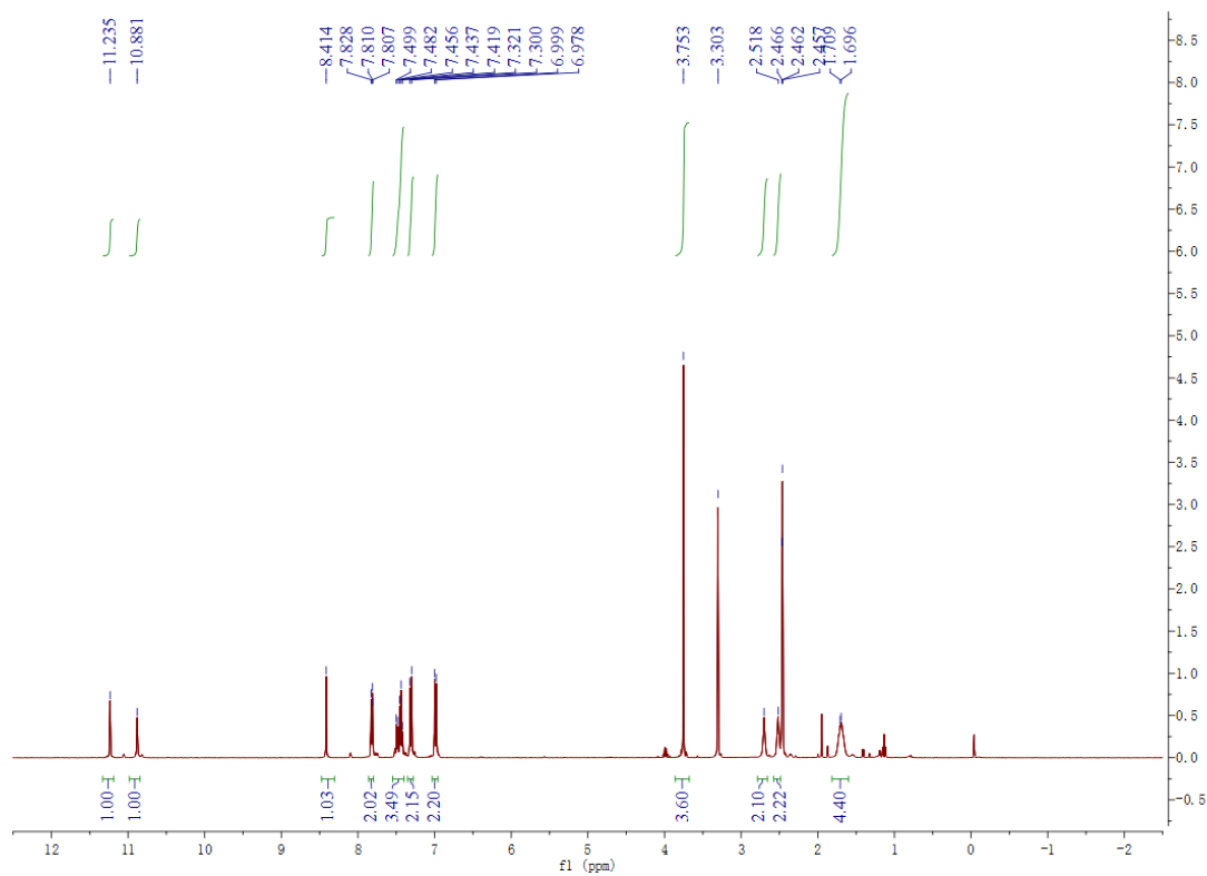
Figure S11. 1 H NMR of compound 7d
