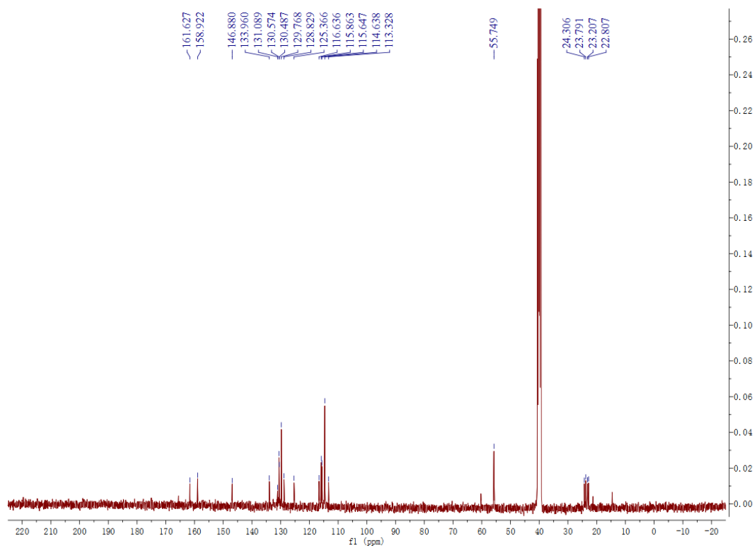
Figure S3. ^{13}\text{C} NMR of compound 7a
