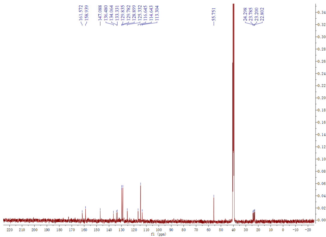
Figure S18. 13 C NMR of compound 7f
