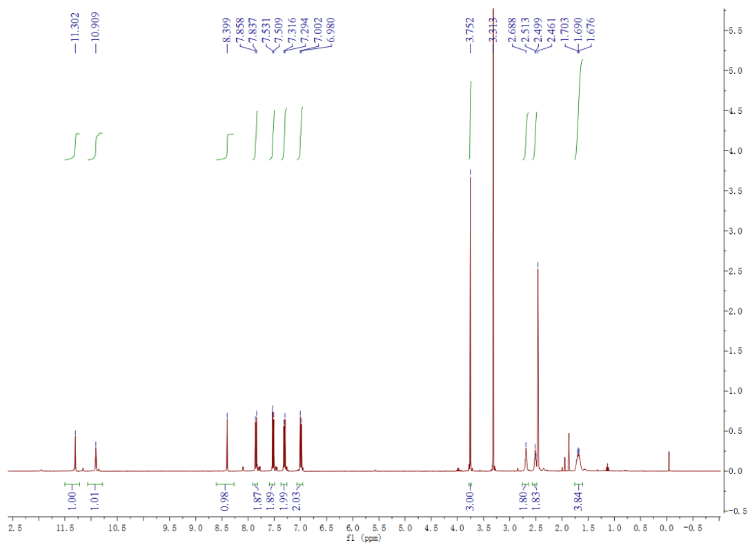
Figure S17. 1 H NMR of compound 7f
