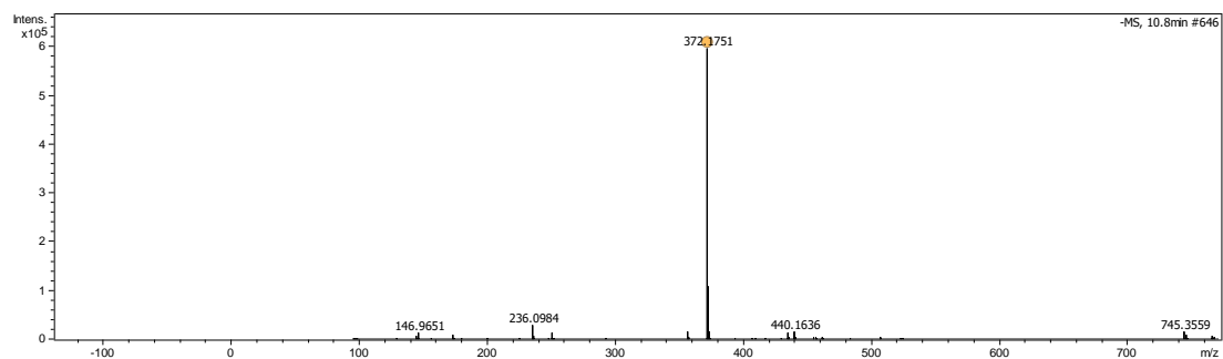
Figure S13. HRMS of compound 7d
