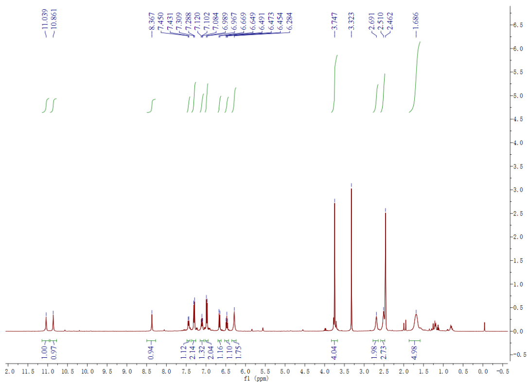
Figure S35. 1 H NMR of compound 7I
