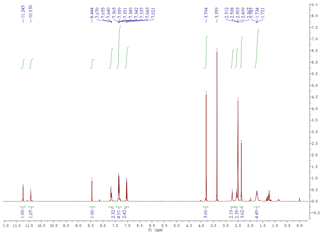
Figure S23. 1 H NMR of compound 7h
