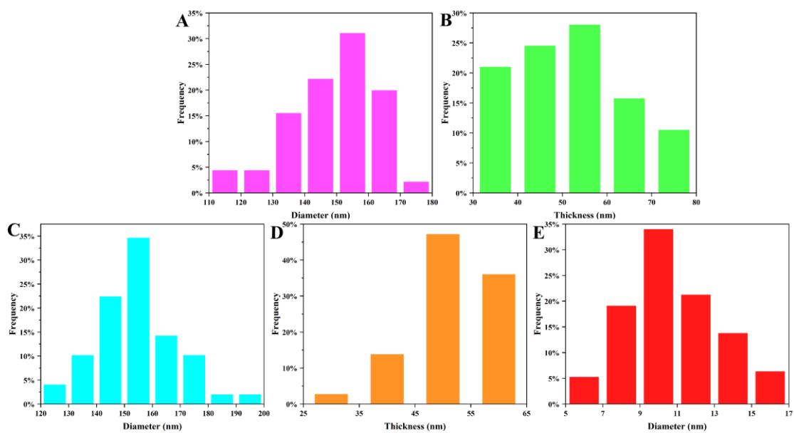
Fig. S1. The size distributions of magnetic \text{Fe}_3\text{O}_4/\alpha\text{-Fe}_2\text{O}_3 heterogeneous nanosheets (A, B), magnetic \text{Fe}_3\text{O}_4/\alpha\text{-Fe}_2\text{O}_3@Au nanocomposites (C, D), and AuNPs (E).
