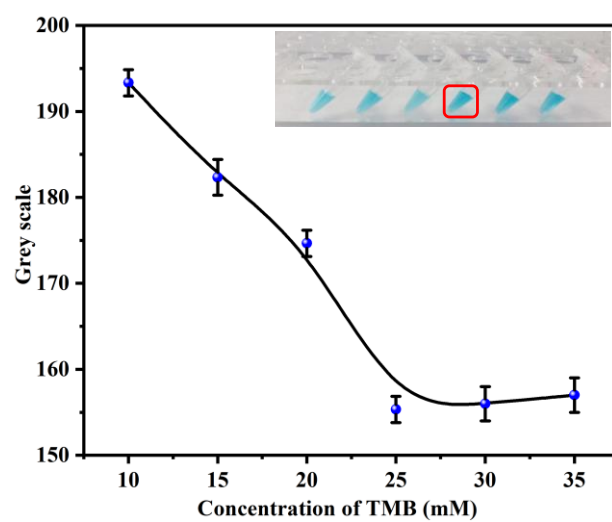
Fig.S3. Optimization of colorimetric mode condition of the concentration of TMB.
