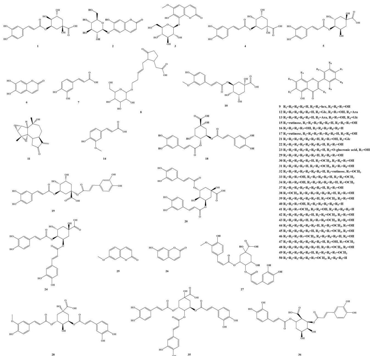
Fig. S1 The chemical structures of the fifty secondary metabolites identified in A. argyi leaves by UPLC-Q/TOF-MS.
