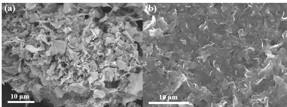
Fig. S3. SEM micrographs of (a) Ti 3 C 2 T x @C and (b) Ti 3 C 2 T x after cyclic stability test.
