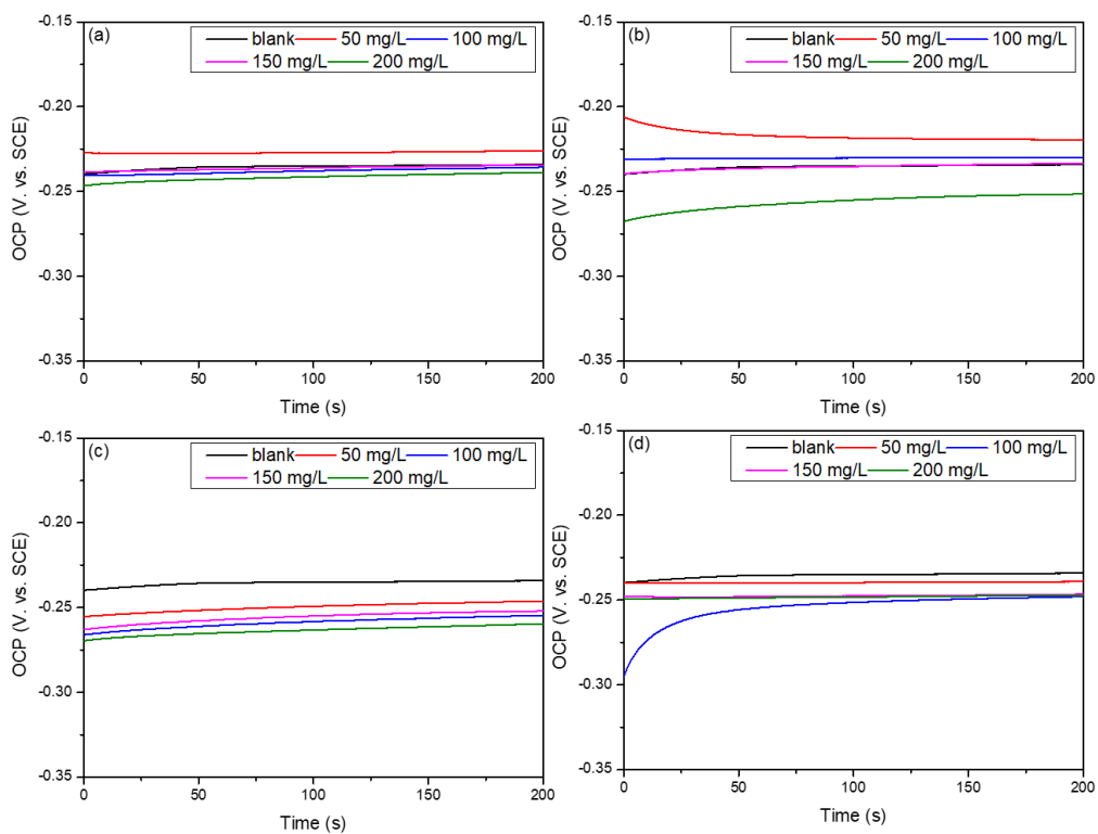
Fig.S1. The variation curve of open circuit potential versus immersion time (a) N-CDs; (b) Cu 1.5 -N-CDs; (c) Cu 3.0 -N-CDs; (d) Cu 6.0 -N-CDs.
