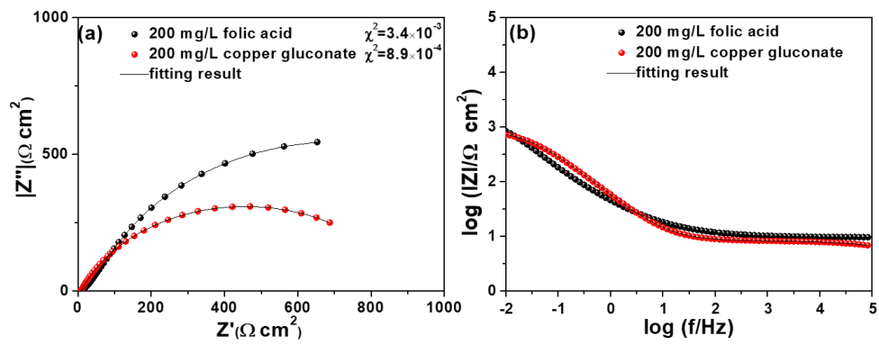
Fig.S2. EIS results of folic acid and copper gluconate (a) Nyquist plots (b) Bode plots.
