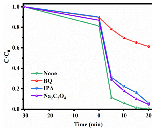
Figure S1 Photocatalytic activities of the C 3 N 4 QDs/MIL-101(Fe)-5 sample for CR degradation with disparate scavengers.
