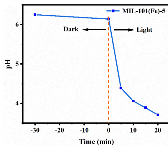
Figure S3 The PH of the photocatalytic degradation of Congo red.
