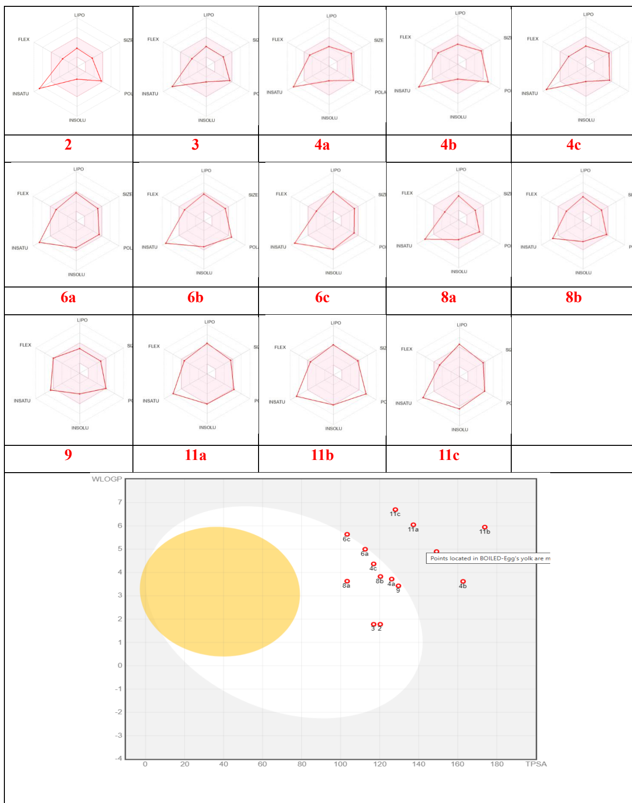
Figure S2. Radar chart and boiled eff figures of the synthesized pyrazine-thiazole analogues.
