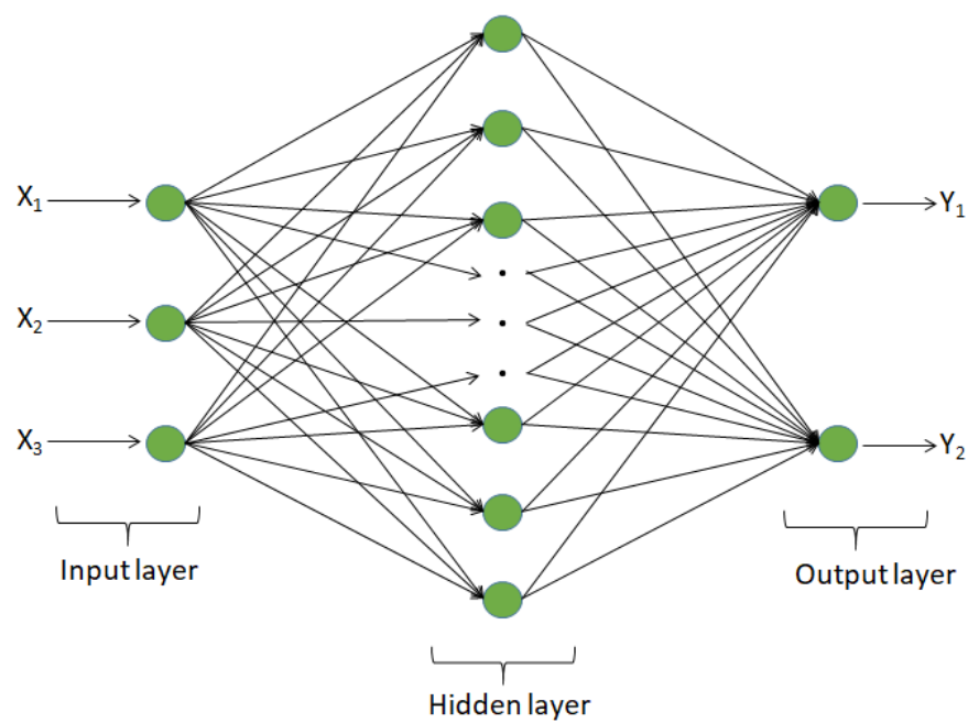
Figure S1 Structure of ANN model, concentration of UCON( X_1 ), concentration of K_2C_4H_4O_6 ( X_2 ), system temperature ( X_3 ), extraction efficiencies of flavonoids ( Y_1 ) and extraction efficiencies of corn silk polysaccharide ( Y_2 ).
