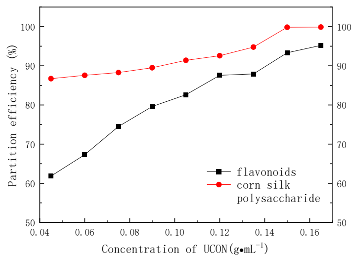
Figure S3 The effect of concentration of UCON on partition efficiency
