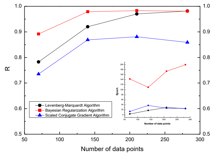
Figure S7 Performances of three algorithms in different scales of datasets
