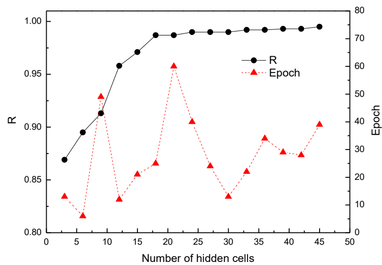
Figure S8 The regression R values and epochs for the ANN model containing different hidden cells
