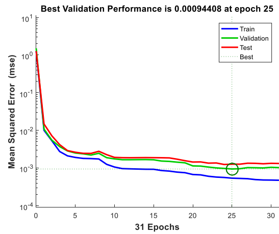
Figure S9 The iterative time and mean squared error
