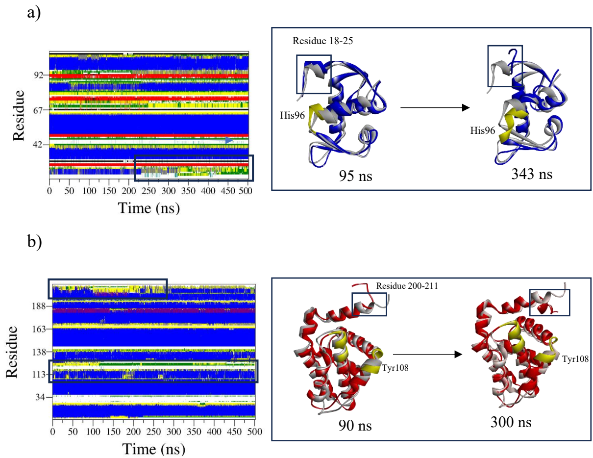
Figure S2 DSSP visual interpretation of (a) C4-MDM2 complex (blue) with its initial structure (grey), and (b) C4-Bcl-2 complex (red) with its initial structure (grey). Yellow color indicates the crucial amino acid in each binding pocket area.
