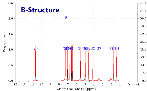
Fig. 2S. H-NMR spectrum of the structures studied in this work.
