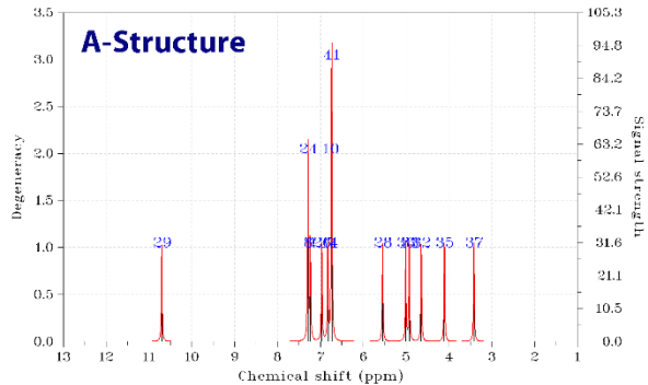
Fig. 2S. H-NMR spectrum of the structures studied in this work.
