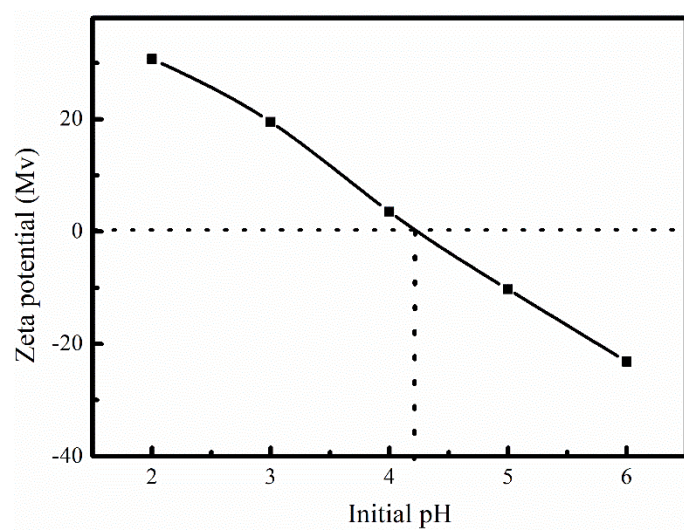
Fig.S1 The zero potential charge of FeNi-BC
