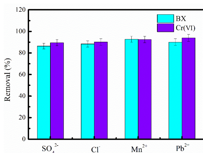
Fig.S2 The coexisting ions can influence the adsorption performance of FeNi-BC for BX and Cr(VI).
