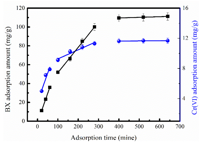
Fig.S3 BX and Cr(VI) adsorption data are fitted using the Intraparticle diffusion model.
