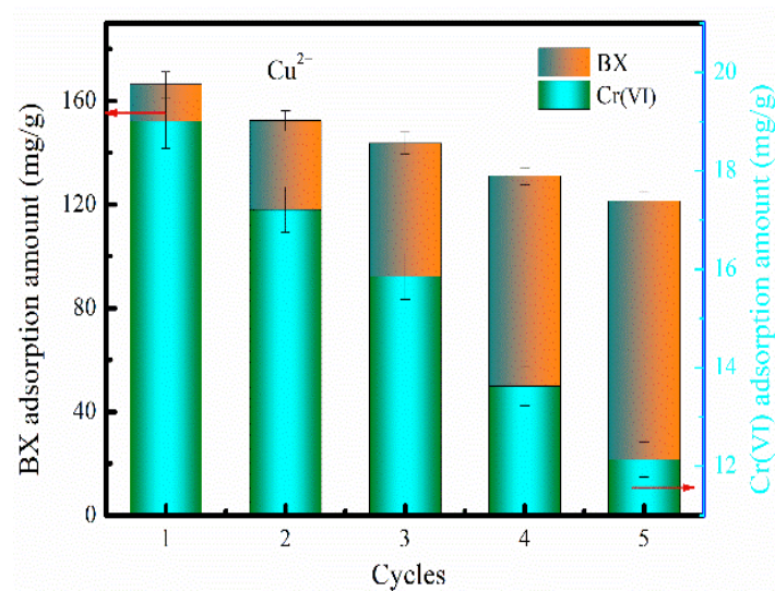
Fig. S4. The recyclability of BX/Cr(VI) adsorption on FeNi-BC
