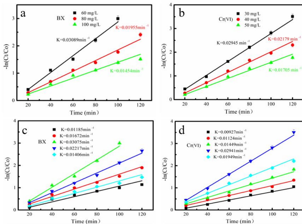
Fig.S5 The relevant kinetic parameters of the different BX (a) and Cr(VI) (b) concentration, different PDS dosage for BX (c) and Cr(VI) (d) in the PDS/FeNi-BC system
