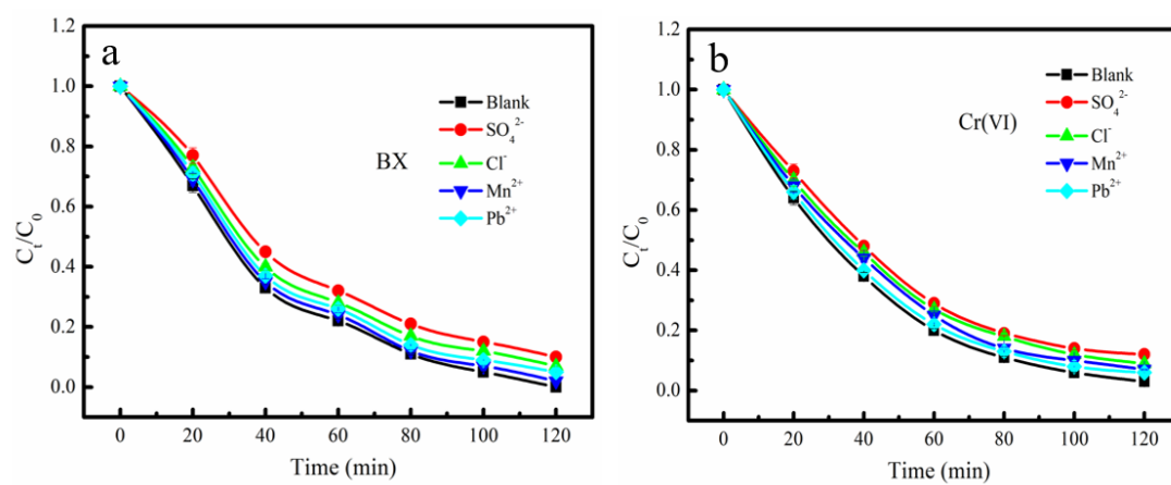
Fig.S6 The influence of \text{SO}_4^{2-} , \text{NO}_3^- , \text{Mn}^{2+} and \text{Pb}^{2+} on BX and Cr(VI) degradation removal.
