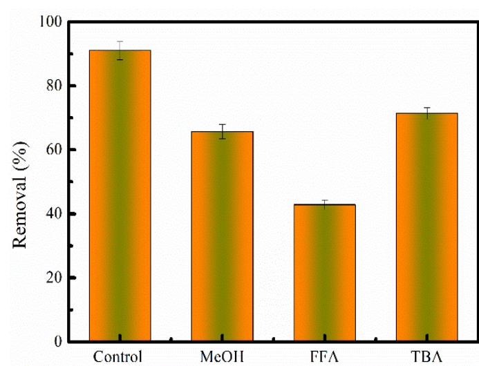
Fig.S8 The free radical quenching for BX degradation.
