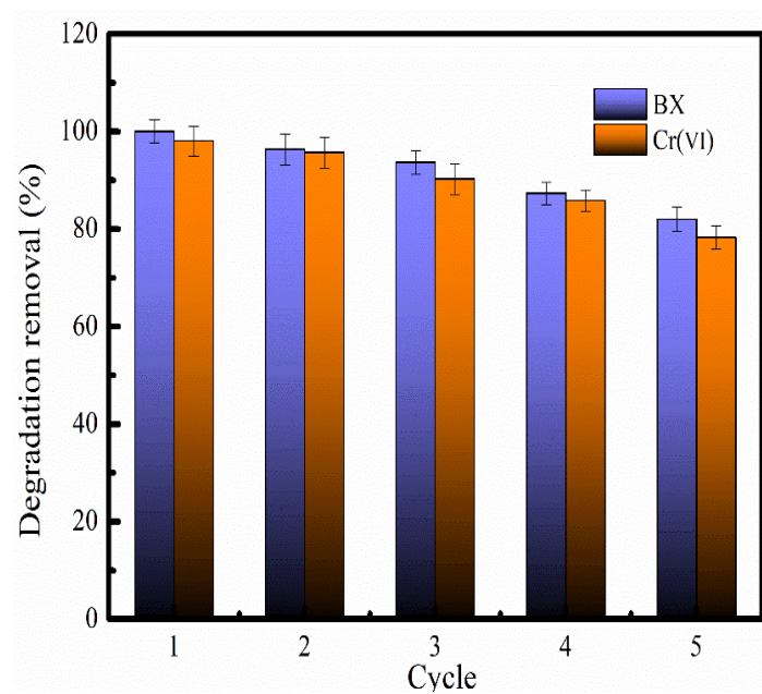
Fig.S9 Reusability degradation performance of the FeNi-BC for BX and Cr(VI)
