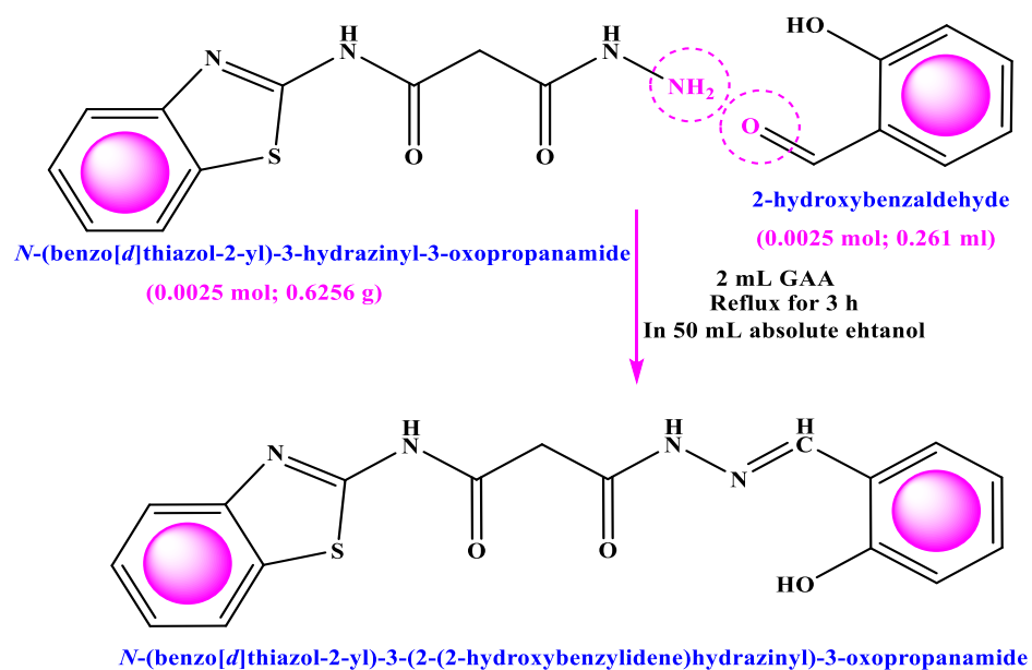
Scheme1S. The outline synthesis of ligand (H 2 BT)
