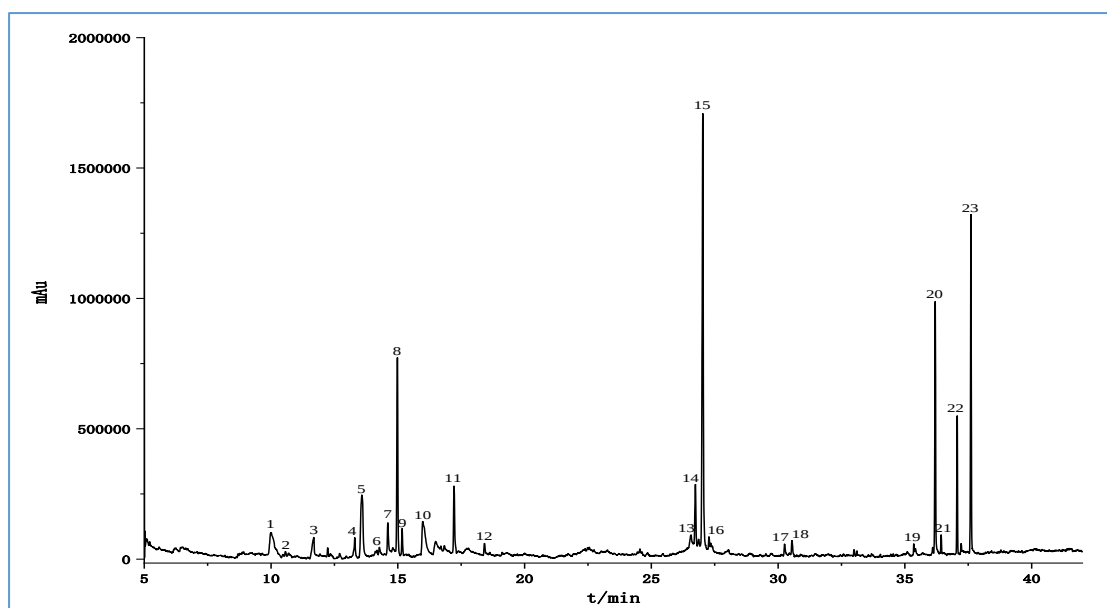
Figure S4. TIC chromatogram by GC-EI-MS qualitative analysis.
