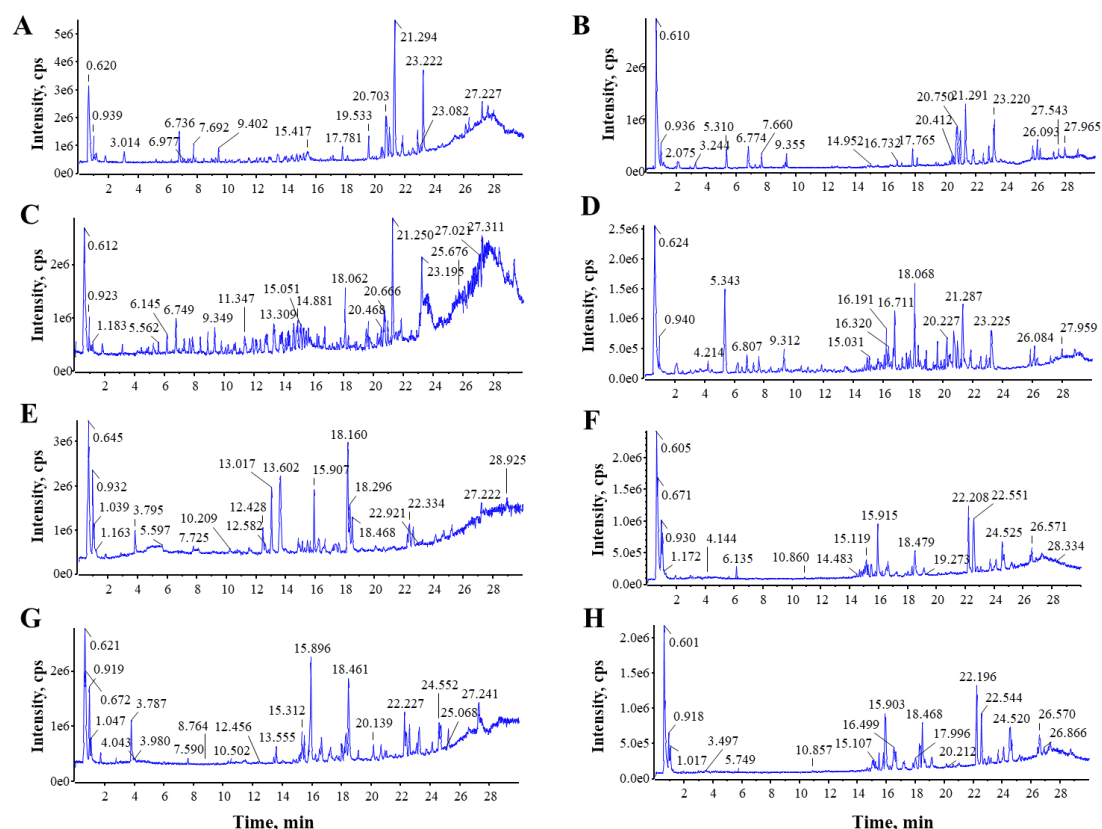
Fig. S3. The total ion chromatogram of SM-LC in vivo by UHPLC-QTOF MS. (A) Plasma sample of control group in positive mode, (B) Plasma sample of control group in negative mode, (C) Plasma sample of SM-LC group in positive mode, (D) Plasma sample of SM-LC group in negative mode, (E) Brain sample of control group in positive mode, (F) Brain sample of control group in negative mode, (G) Brain sample of SM-LC group in positive mode, (H) Brain sample of SM-LC group in negative mode.
