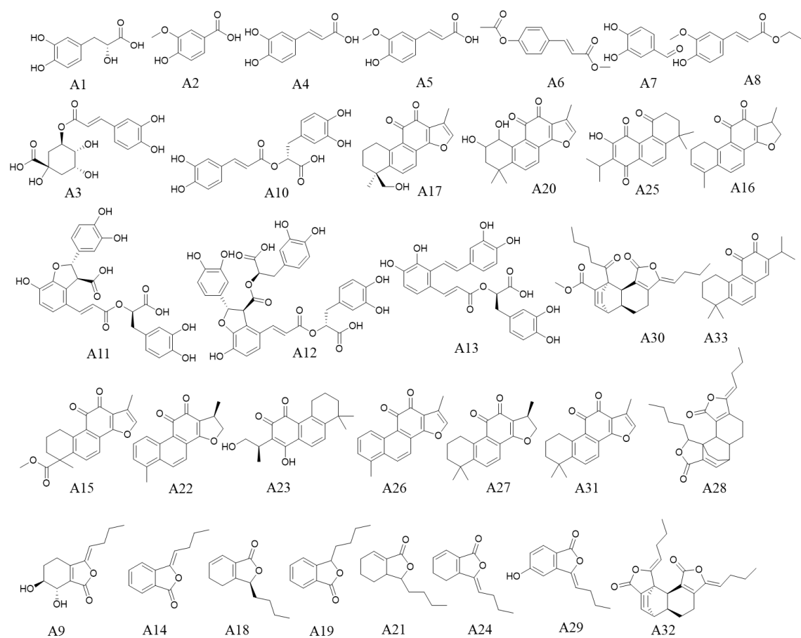
Fig. S4. Chemical structures of 33 prototypes of SM-LC in vivo .
