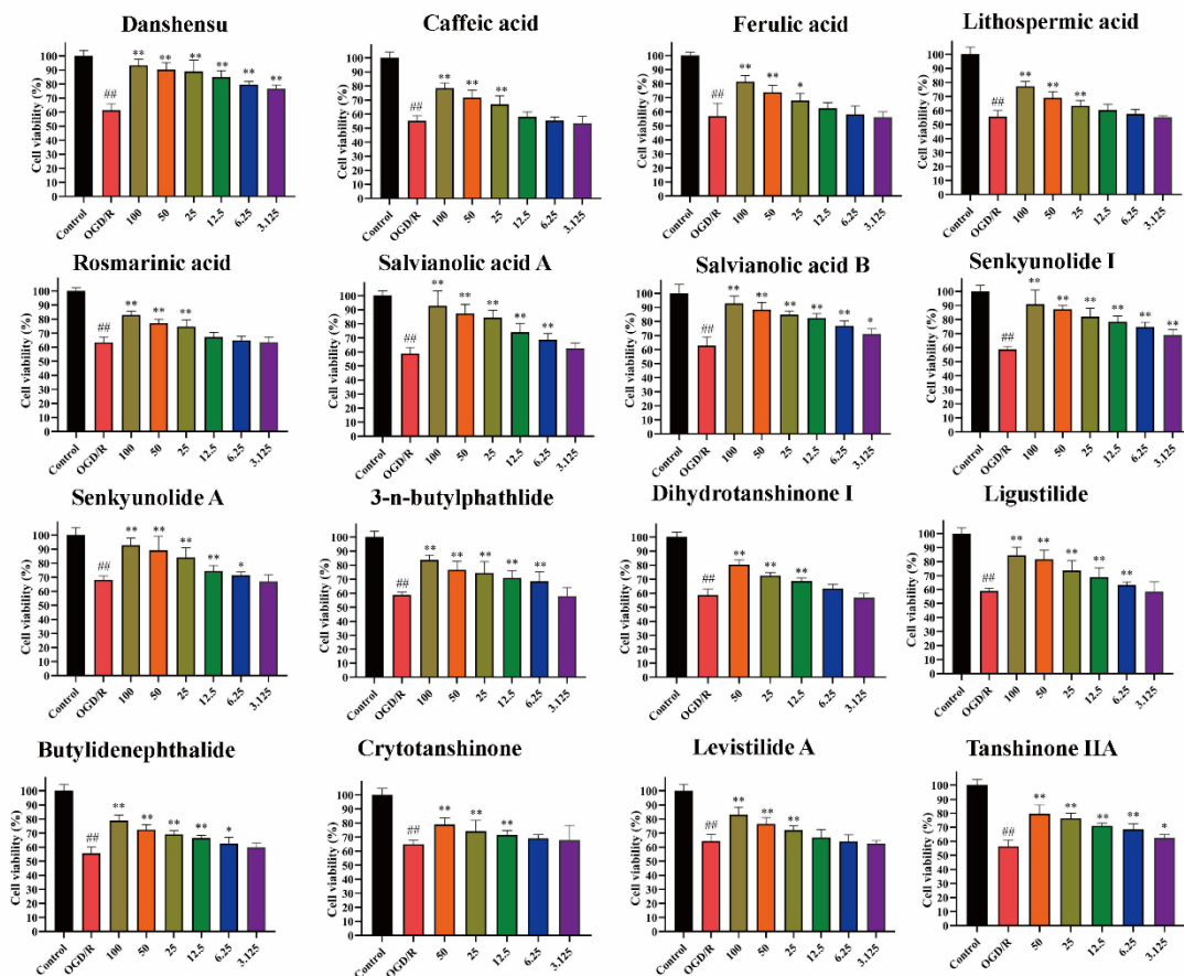
Fig. S6. The effects of 16 prototypes on the cell viability of BEND.3 cells injury model. Data was presented as mean \pm SD (n = 6), ^{##}P < 0.01 compared to control group; while ^{*}P < 0.05 , ^{**}P < 0.01 compared to OGD/R group.
